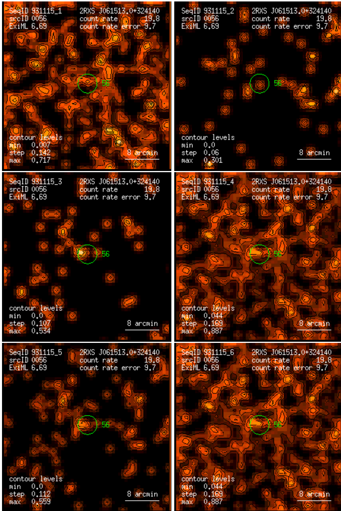
Figure 56: RASS 931115: detection 0056: band rate images, Gaussian filter: (1) PSPC channels 11 – 41, (2) 52 – 90, (3) 91 – 201, (4) 11 – 235, (5) 52 – 201, (6) 11 – 201. Broad band rates in counts/ks. Band rate contour levels in counts/ks/arcmin 2 .
