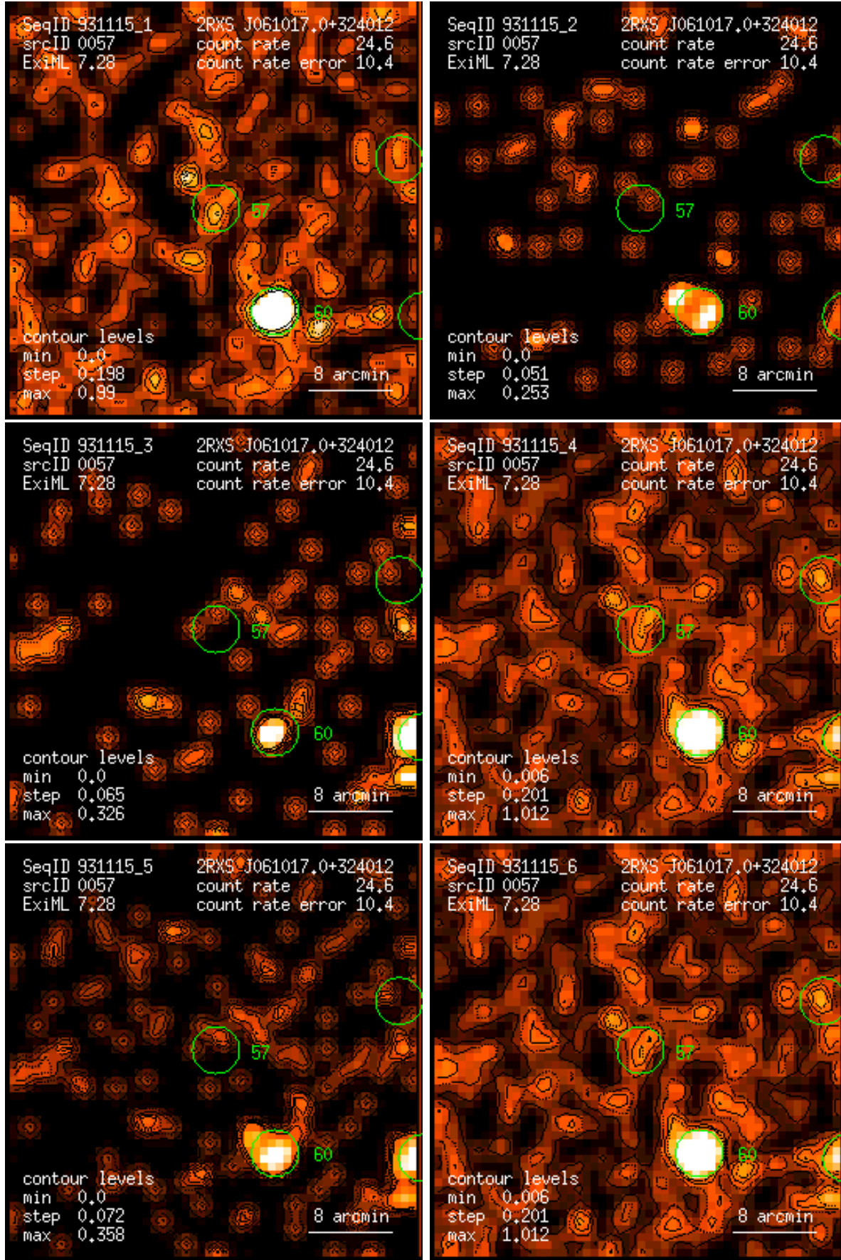
Figure 57: RASS 931115: detection 0057: band rate images, Gaussian filter: (1) PSPC channels 11 – 41, (2) 52 – 90, (3) 91 – 201, (4) 11 – 235, (5) 52 – 201, (6) 11 – 201. Broad band rates in counts/ks. Band rate contour levels in counts/ks/arcmin 2 .
