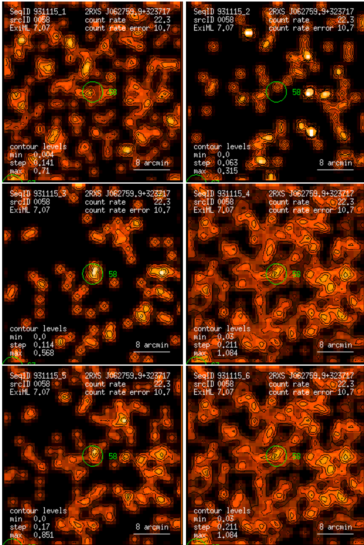
Figure 58: RASS 931115: detection 0058: band rate images, Gaussian filter: (1) PSPC channels 11 – 41, (2) 52 – 90, (3) 91 – 201, (4) 11 – 235, (5) 52 – 201, (6) 11 – 201. Broad band rates in counts/ks. Band rate contour levels in counts/ks/arcmin 2 .
