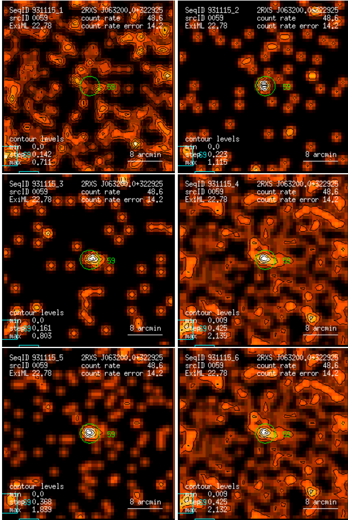
Figure 59: RASS 931115: detection 0059: band rate images, Gaussian filter: (1) PSPC channels 11 – 41, (2) 52 – 90, (3) 91 – 201, (4) 11 – 235, (5) 52 – 201, (6) 11 – 201. Broad band rates in counts/ks. Band rate contour levels in counts/ks/arcmin 2 .
