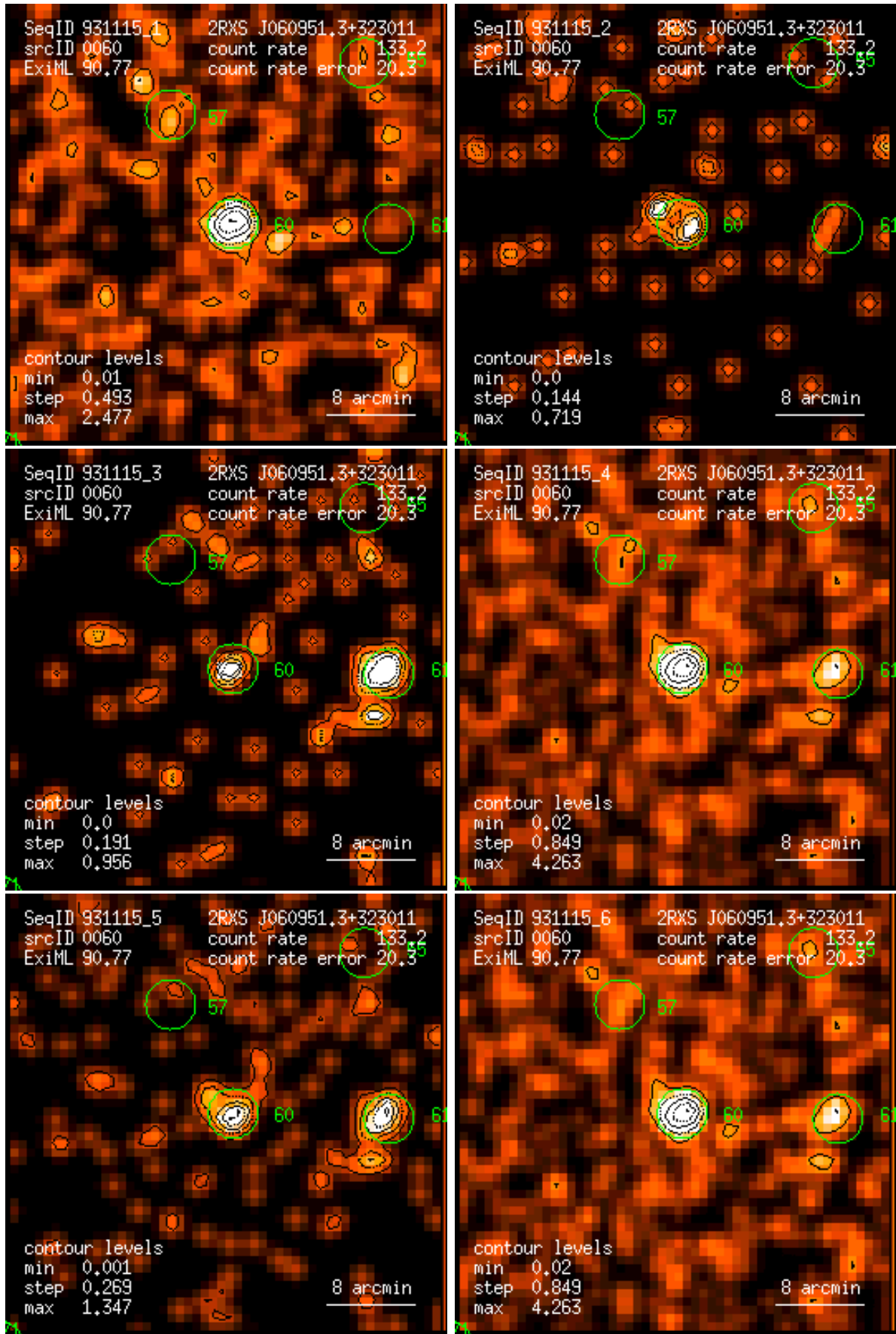
Figure 60: RASS 931115: detection 0060: band rate images, Gaussian filter: (1) PSPC channels 11 – 41, (2) 52 – 90, (3) 91 – 201, (4) 11 – 235, (5) 52 – 201, (6) 11 – 201. Broad band rates in counts/ks. Band rate contour levels in counts/ks/arcmin 2 .
