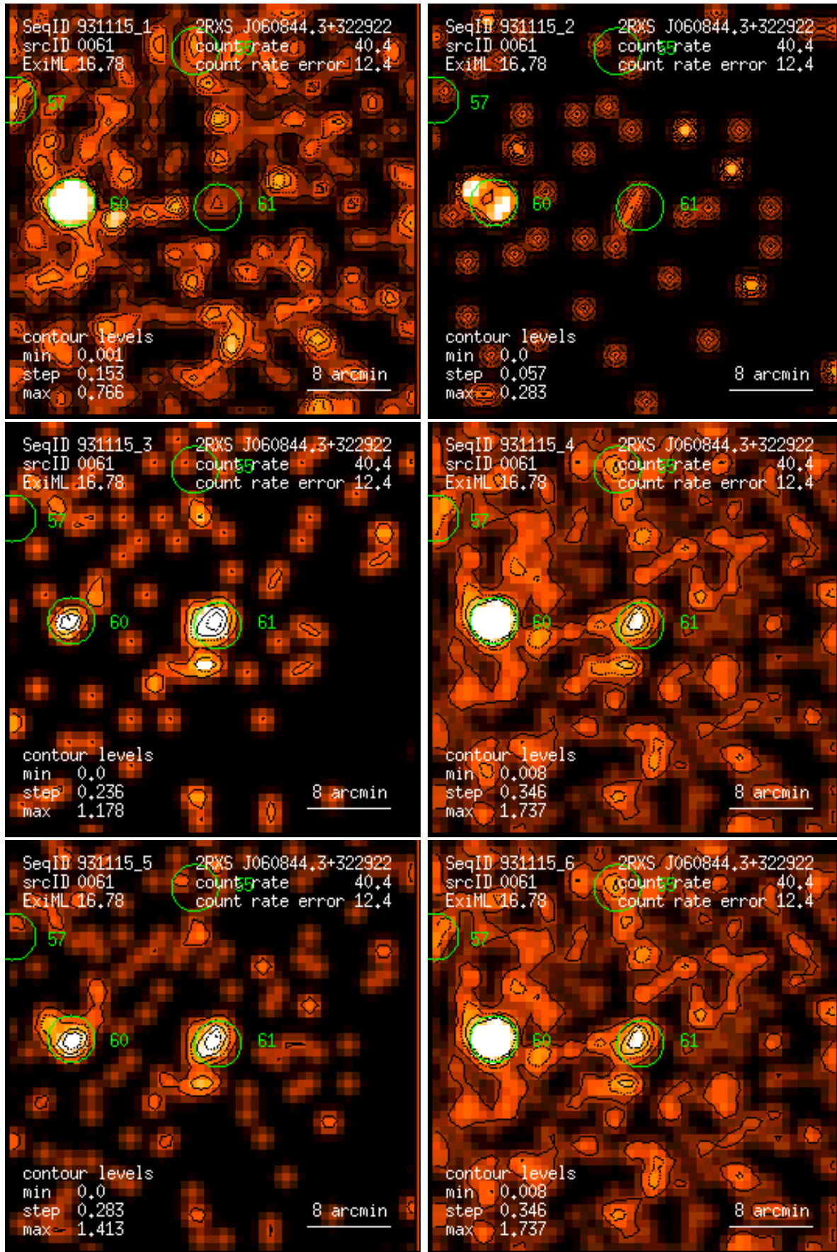
Figure 61: RASS 931115: detection 0061: band rate images, Gaussian filter: (1) PSPC channels 11 – 41, (2) 52 – 90, (3) 91 – 201, (4) 11 – 235, (5) 52 – 201, (6) 11 – 201. Broad band rates in counts/ks. Band rate contour levels in counts/ks/arcmin 2 .
