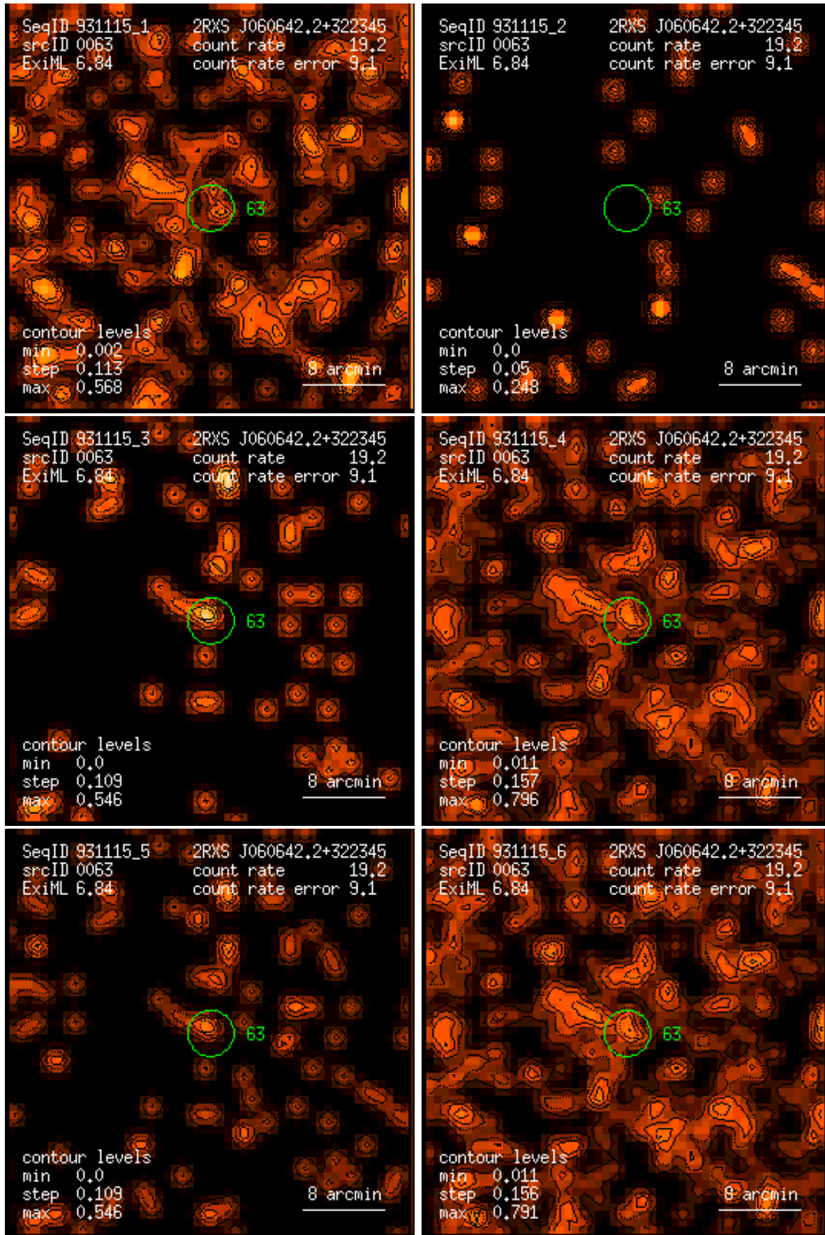
Figure 63: RASS 931115: detection 0063: band rate images, Gaussian filter: (1) PSPC channels 11 – 41, (2) 52 – 90, (3) 91 – 201, (4) 11 – 235, (5) 52 – 201, (6) 11 – 201. Broad band rates in counts/ks. Band rate contour levels in counts/ks/arcmin 2 .
