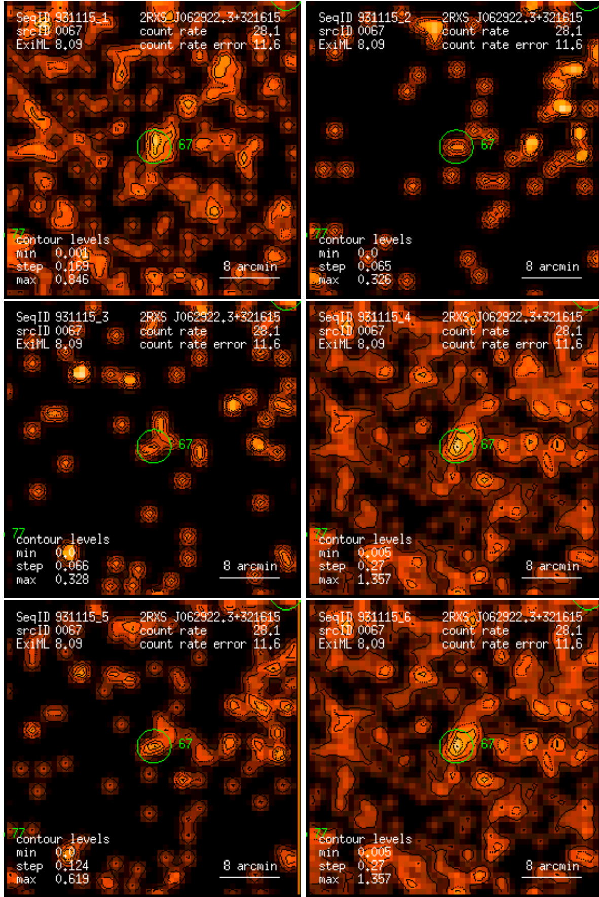
Figure 67: RASS 931115: detection 0067: band rate images, Gaussian filter: (1) PSPC channels 11 – 41, (2) 52 – 90, (3) 91 – 201, (4) 11 – 235, (5) 52 – 201, (6) 11 – 201. Broad band rates in counts/ks. Band rate contour levels in counts/ks/arcmin 2 .
