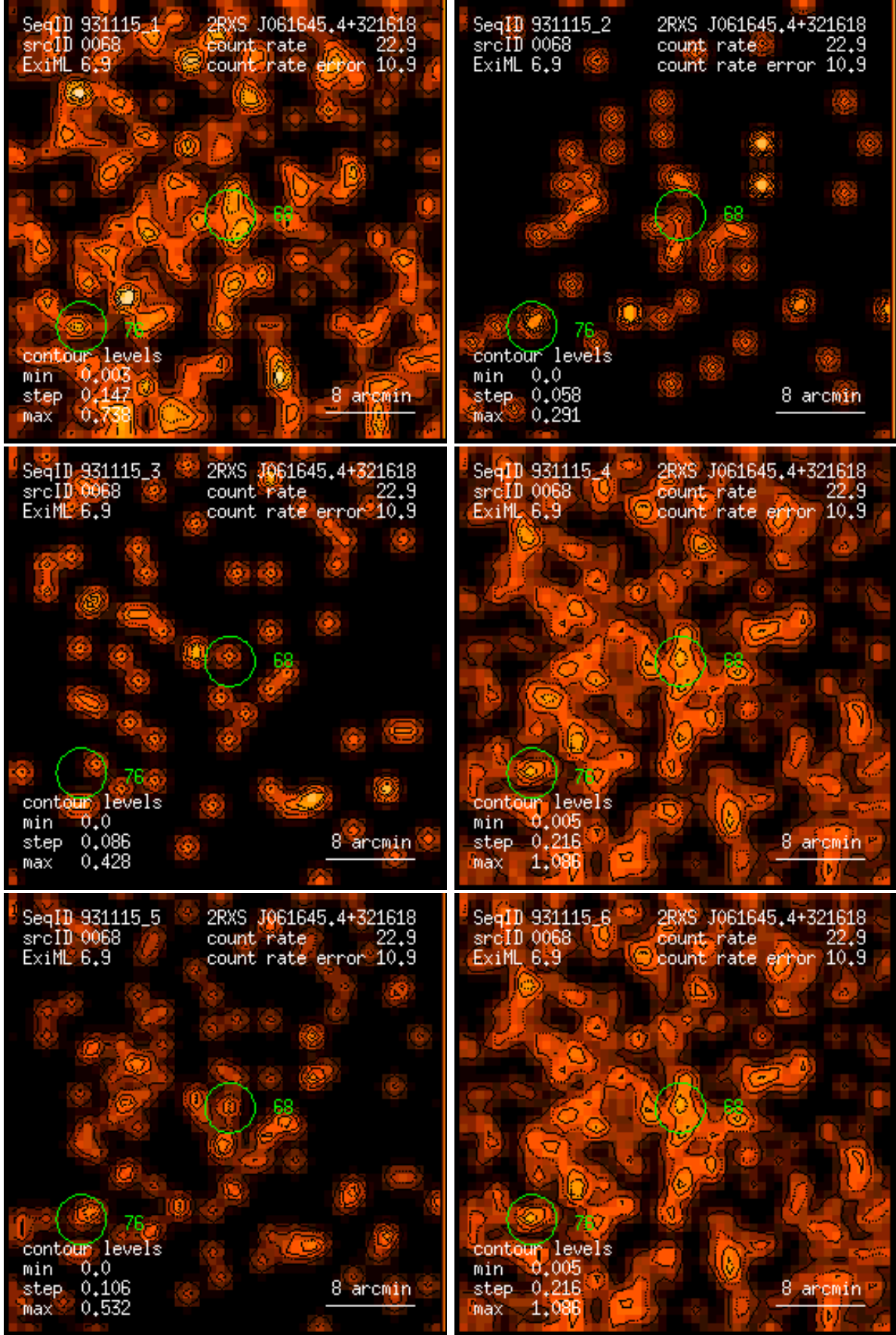
Figure 68: RASS 931115: detection 0068: band rate images, Gaussian filter: (1) PSPC channels 11 – 41, (2) 52 – 90, (3) 91 – 201, (4) 11 – 235, (5) 52 – 201, (6) 11 – 201. Broad band rates in counts/ks. Band rate contour levels in counts/ks/arcmin 2 .
