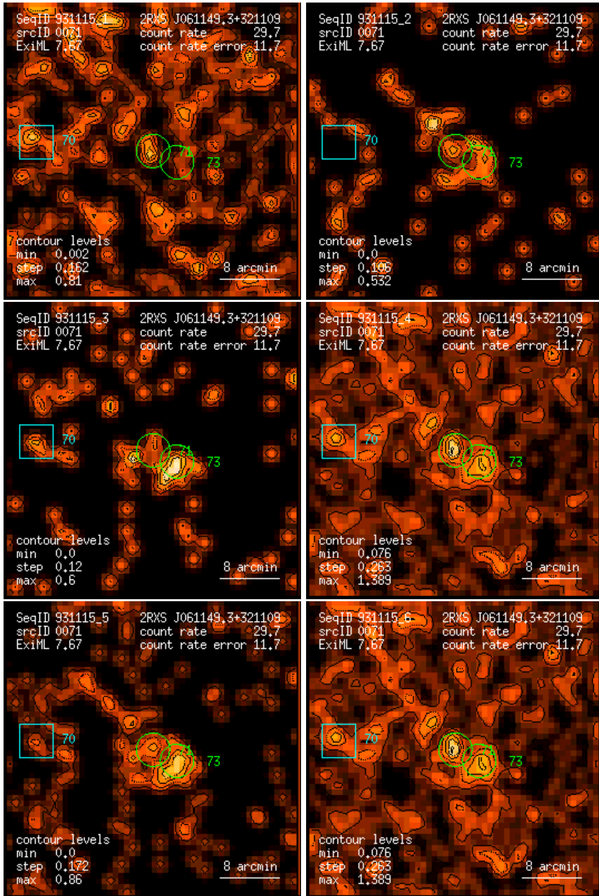
Figure 71: RASS 931115: detection 0071: band rate images, Gaussian filter: (1) PSPC channels 11 – 41, (2) 52 – 90, (3) 91 – 201, (4) 11 – 235, (5) 52 – 201, (6) 11 – 201. Broad band rates in counts/ks. Band rate contour levels in counts/ks/arcmin 2 .
