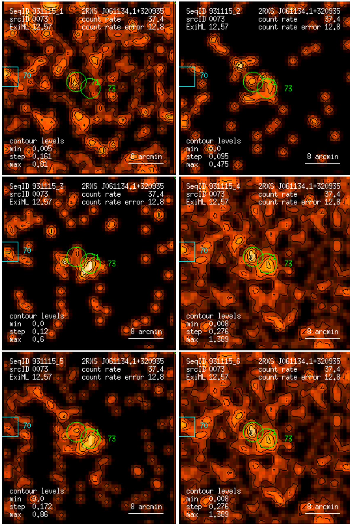
Figure 73: RASS 931115: detection 0073: band rate images, Gaussian filter: (1) PSPC channels 11 – 41, (2) 52 – 90, (3) 91 – 201, (4) 11 – 235, (5) 52 – 201, (6) 11 – 201. Broad band rates in counts/ks. Band rate contour levels in counts/ks/arcmin 2 .
