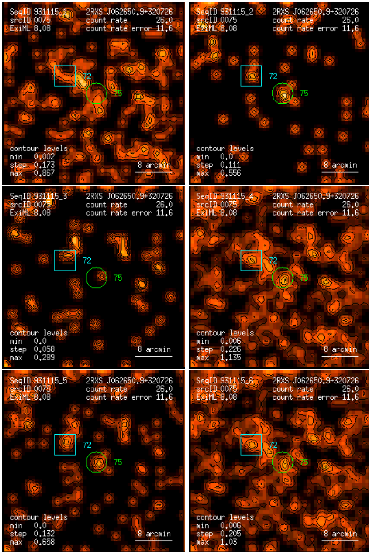
Figure 75: RASS 931115: detection 0075: band rate images, Gaussian filter: (1) PSPC channels 11 – 41, (2) 52 – 90, (3) 91 – 201, (4) 11 – 235, (5) 52 – 201, (6) 11 – 201. Broad band rates in counts/ks. Band rate contour levels in counts/ks/arcmin 2 .
