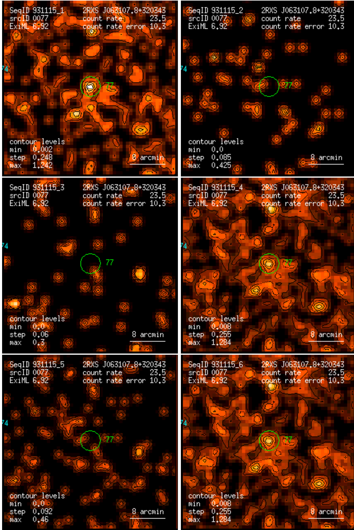
Figure 77: RASS 931115: detection 0077: band rate images, Gaussian filter: (1) PSPC channels 11 – 41, (2) 52 – 90, (3) 91 – 201, (4) 11 – 235, (5) 52 – 201, (6) 11 – 201. Broad band rates in counts/ks. Band rate contour levels in counts/ks/arcmin 2 .
