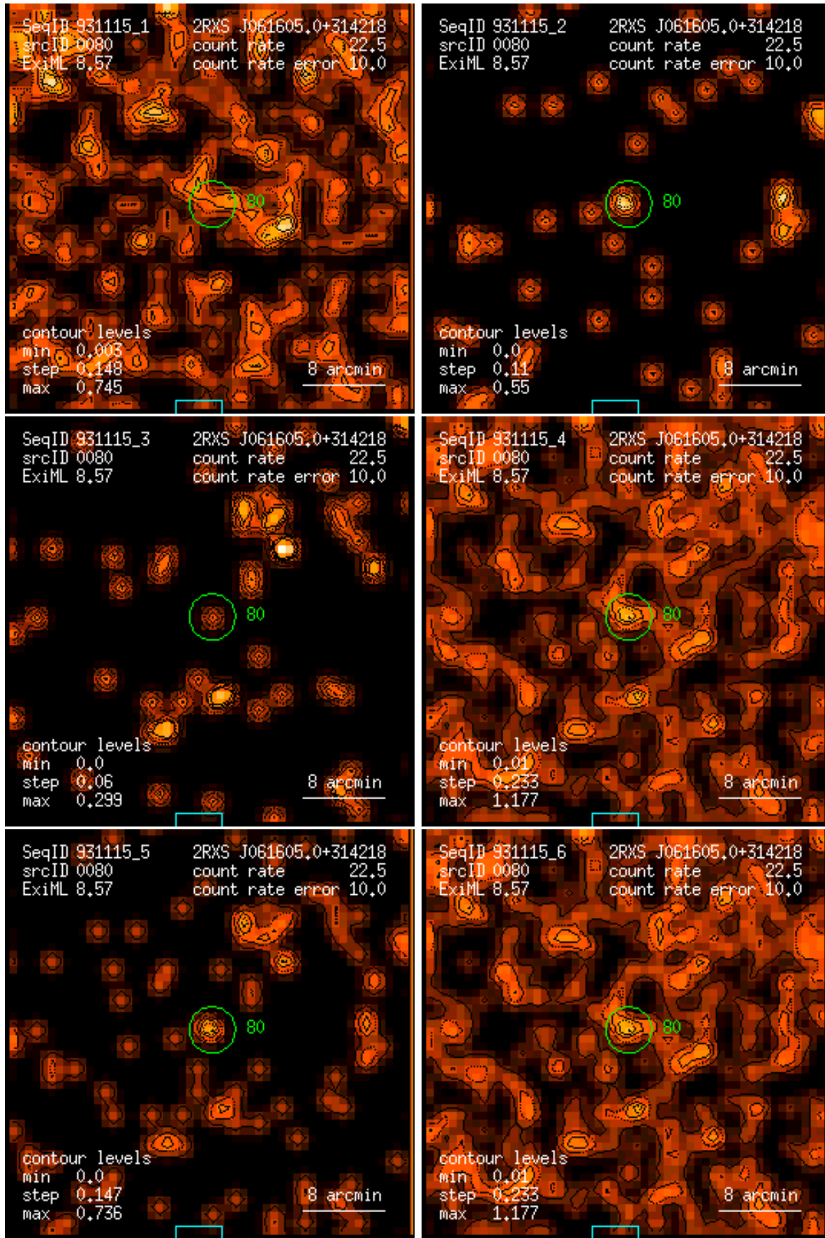
Figure 80: RASS 931115: detection 0080: band rate images, Gaussian filter: (1) PSPC channels 11 – 41, (2) 52 – 90, (3) 91 – 201, (4) 11 – 235, (5) 52 – 201, (6) 11 – 201. Broad band rates in counts/ks. Band rate contour levels in counts/ks/arcmin 2 .
