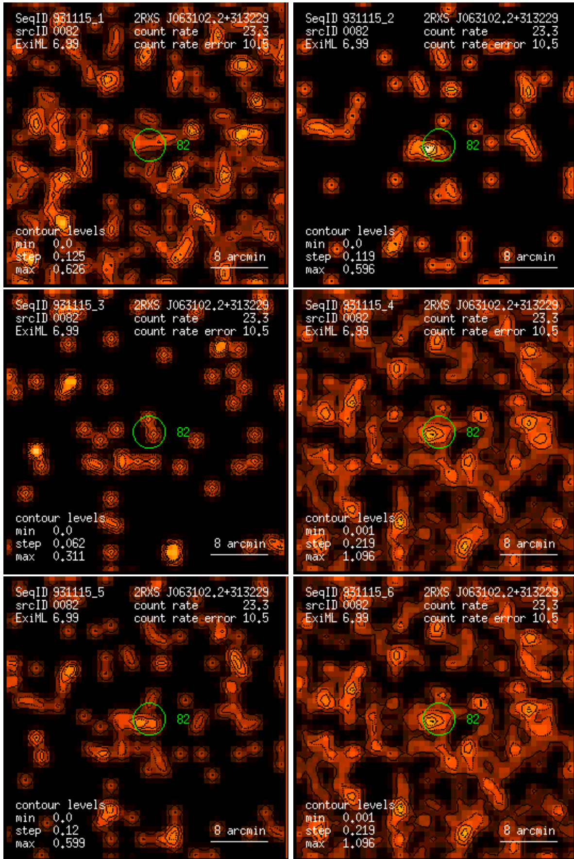
Figure 82: RASS 931115: detection 0082: band rate images, Gaussian filter: (1) PSPC channels 11 – 41, (2) 52 – 90, (3) 91 – 201, (4) 11 – 235, (5) 52 – 201, (6) 11 – 201. Broad band rates in counts/ks. Band rate contour levels in counts/ks/arcmin 2 .
