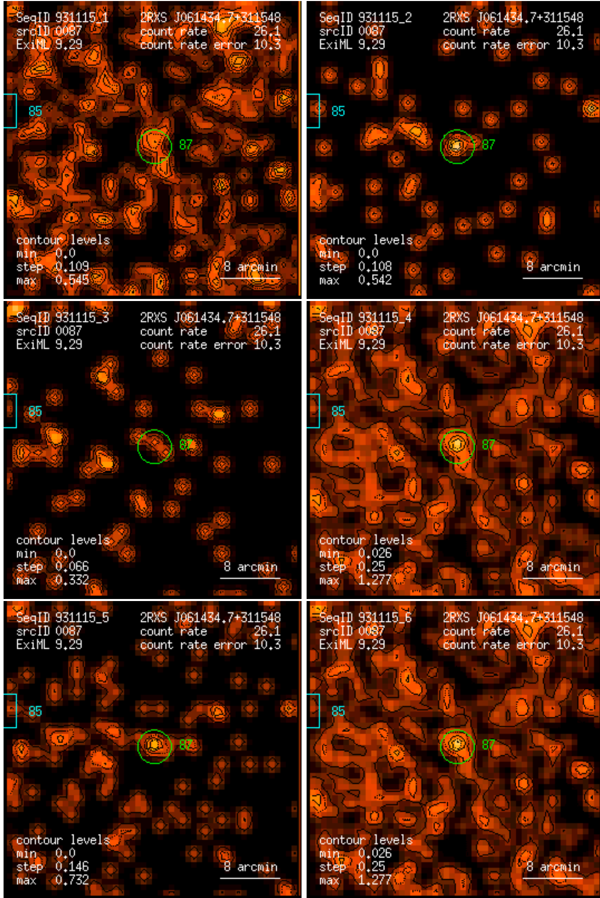
Figure 87: RASS 931115: detection 0087: band rate images, Gaussian filter: (1) PSPC channels 11 – 41, (2) 52 – 90, (3) 91 – 201, (4) 11 – 235, (5) 52 – 201, (6) 11 – 201. Broad band rates in counts/ks. Band rate contour levels in counts/ks/arcmin 2 .
