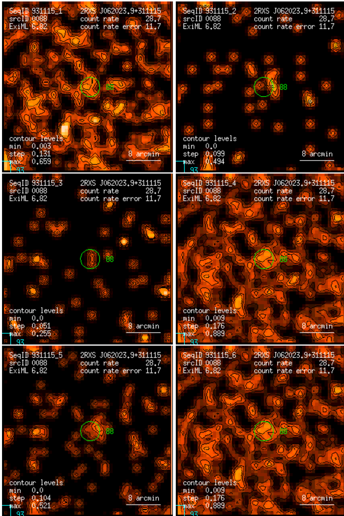
Figure 88: RASS 931115: detection 0088: band rate images, Gaussian filter: (1) PSPC channels 11 – 41, (2) 52 – 90, (3) 91 – 201, (4) 11 – 235, (5) 52 – 201, (6) 11 – 201. Broad band rates in counts/ks. Band rate contour levels in counts/ks/arcmin 2 .
