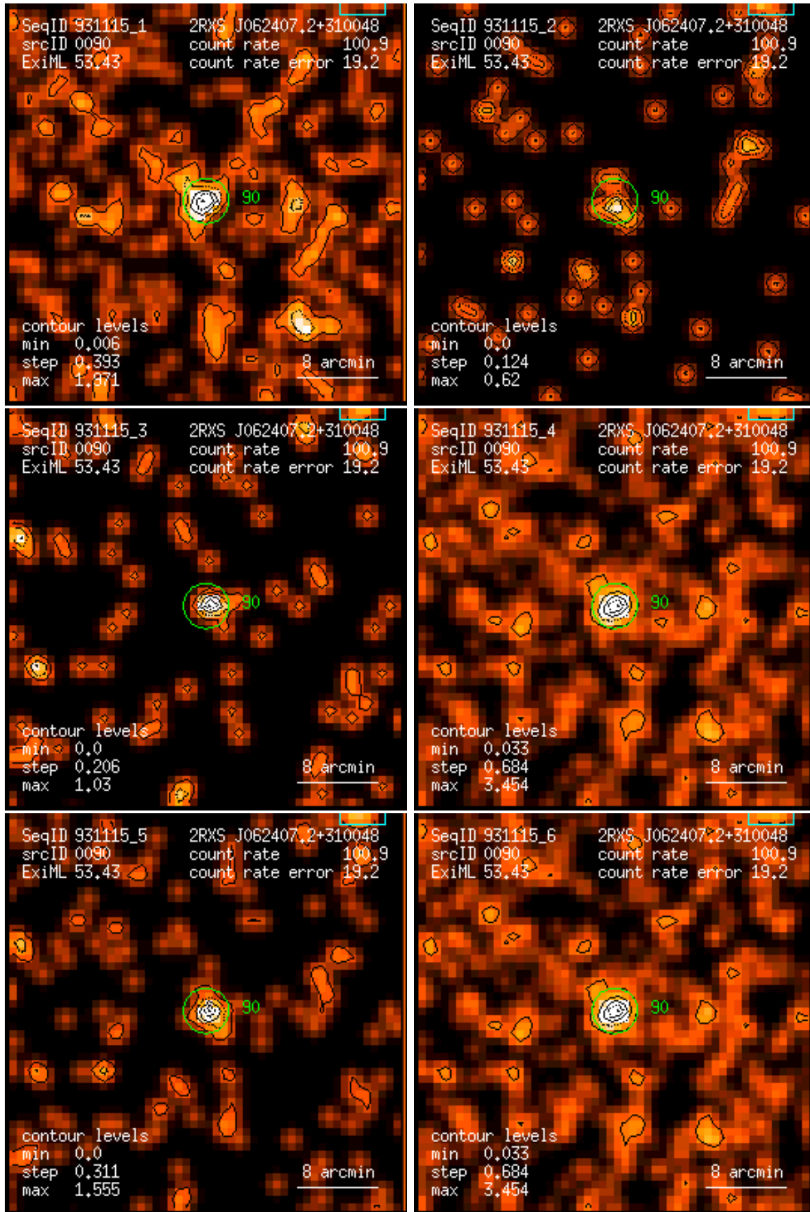
Figure 90: RASS 931115: detection 0090: band rate images, Gaussian filter: (1) PSPC channels 11 – 41, (2) 52 – 90, (3) 91 – 201, (4) 11 – 235, (5) 52 – 201, (6) 11 – 201. Broad band rates in counts/ks. Band rate contour levels in counts/ks/arcmin 2 .
