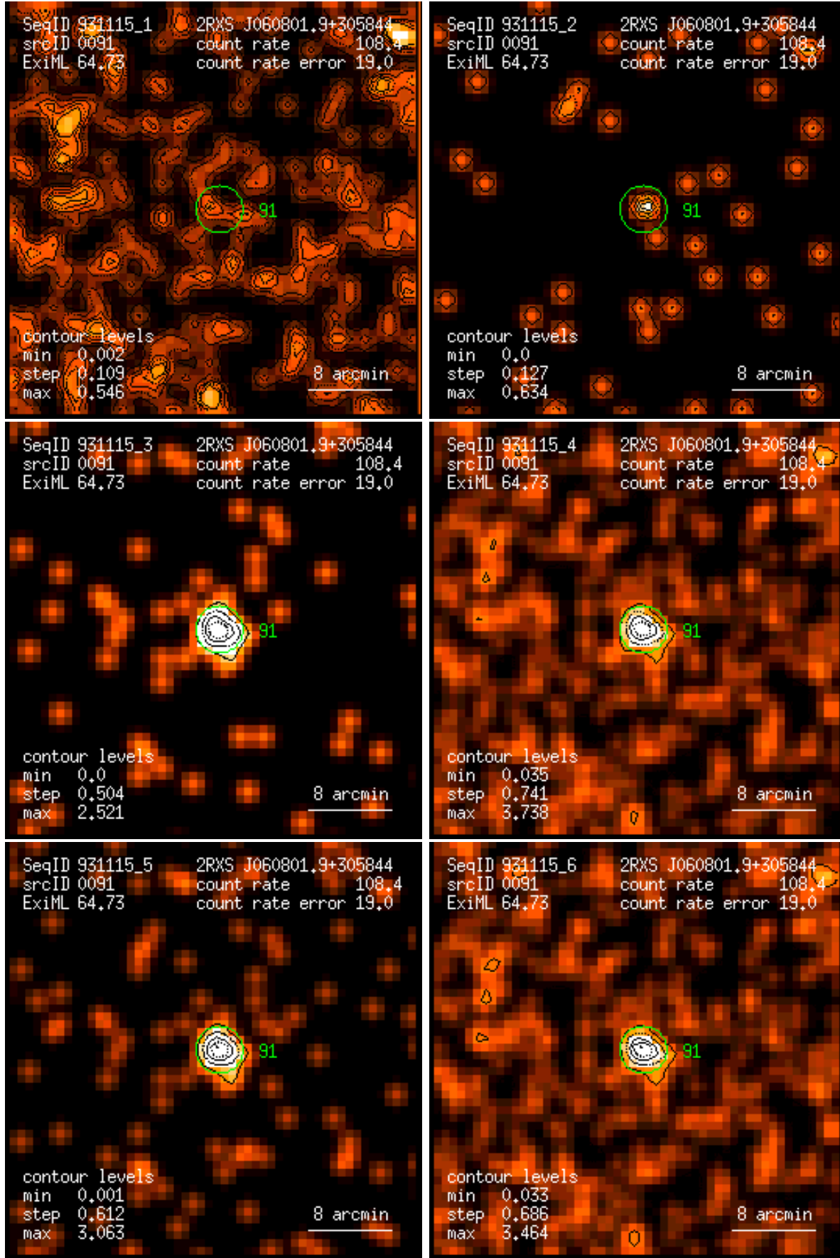
Figure 91: RASS 931115: detection 0091: band rate images, Gaussian filter: (1) PSPC channels 11 – 41, (2) 52 – 90, (3) 91 – 201, (4) 11 – 235, (5) 52 – 201, (6) 11 – 201. Broad band rates in counts/ks. Band rate contour levels in counts/ks/arcmin 2 .
