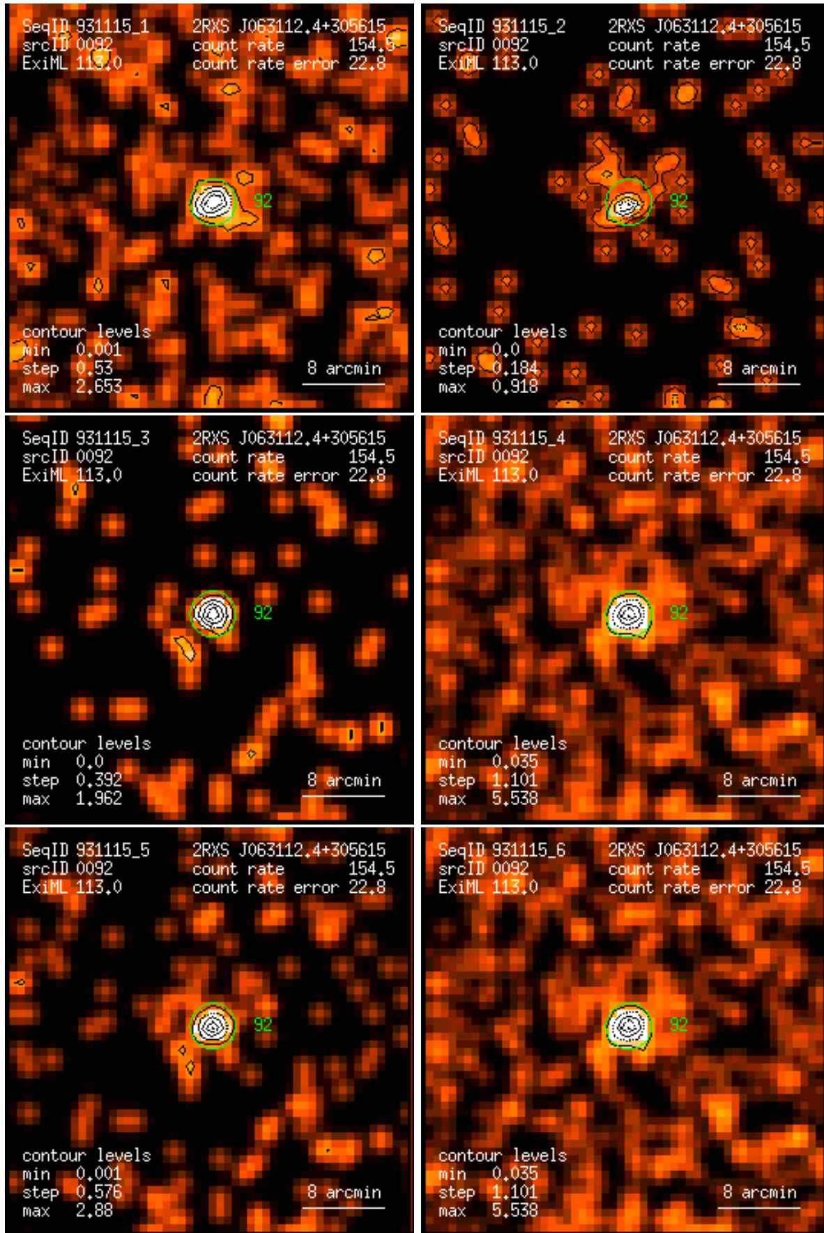
Figure 92: RASS 931115: detection 0092: band rate images, Gaussian filter: (1) PSPC channels 11 – 41, (2) 52 – 90, (3) 91 – 201, (4) 11 – 235, (5) 52 – 201, (6) 11 – 201. Broad band rates in counts/ks. Band rate contour levels in counts/ks/arcmin 2 .
