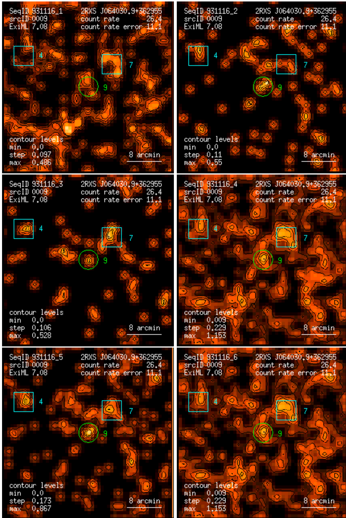
Figure 9: RASS 931116: detection 0009: band rate images, Gaussian filter: (1) PSPC channels 11 – 41, (2) 52 – 90, (3) 91 – 201, (4) 11 – 235, (5) 52 – 201, (6) 11 – 201. Broad band rates in counts/ks. Band rate contour levels in counts/ks/arcmin 2 .
