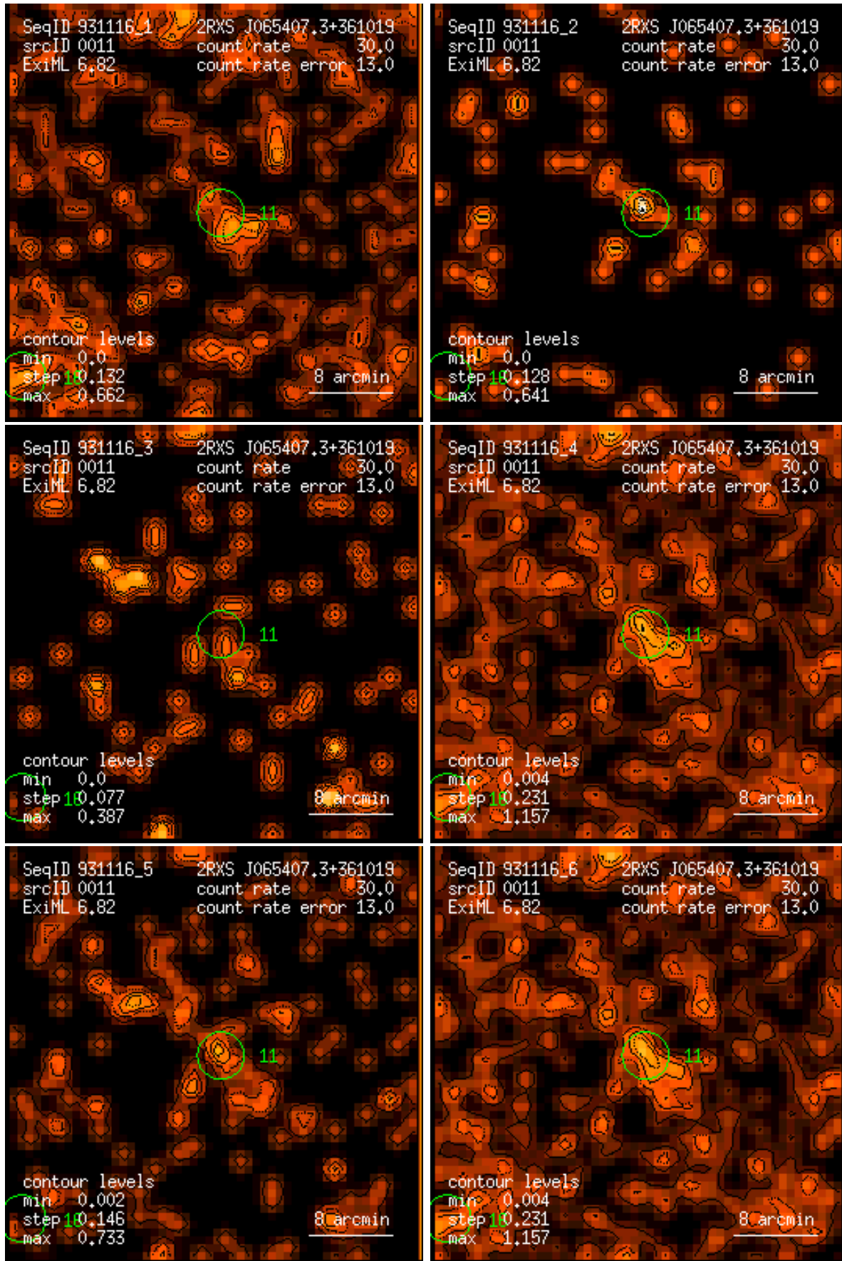
Figure 11: RASS 931116: detection 0011: band rate images, Gaussian filter: (1) PSPC channels 11 – 41, (2) 52 – 90, (3) 91 – 201, (4) 11 – 235, (5) 52 – 201, (6) 11 – 201. Broad band rates in counts/ks. Band rate contour levels in counts/ks/arcmin 2 .
