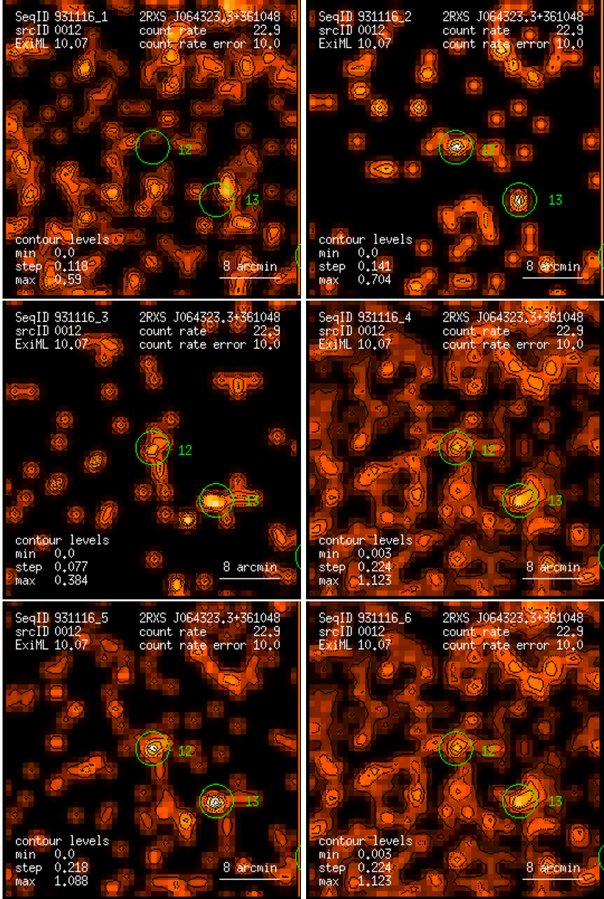
Figure 12: RASS 931116: detection 0012: band rate images, Gaussian filter: (1) PSPC channels 11 – 41, (2) 52 – 90, (3) 91 – 201, (4) 11 – 235, (5) 52 – 201, (6) 11 – 201. Broad band rates in counts/ks. Band rate contour levels in counts/ks/arcmin 2 .
