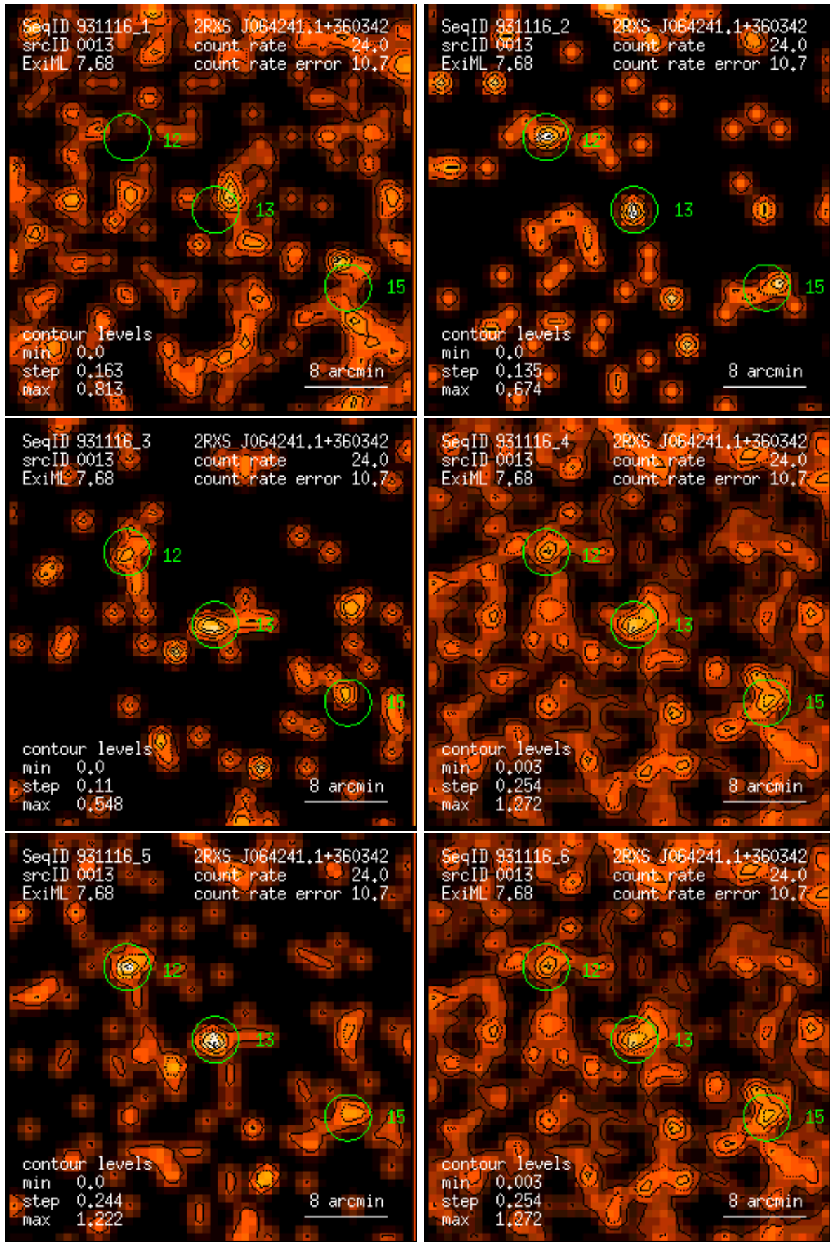
Figure 13: RASS 931116: detection 0013: band rate images, Gaussian filter: (1) PSPC channels 11 – 41, (2) 52 – 90, (3) 91 – 201, (4) 11 – 235, (5) 52 – 201, (6) 11 – 201. Broad band rates in counts/ks. Band rate contour levels in counts/ks/arcmin 2 .
