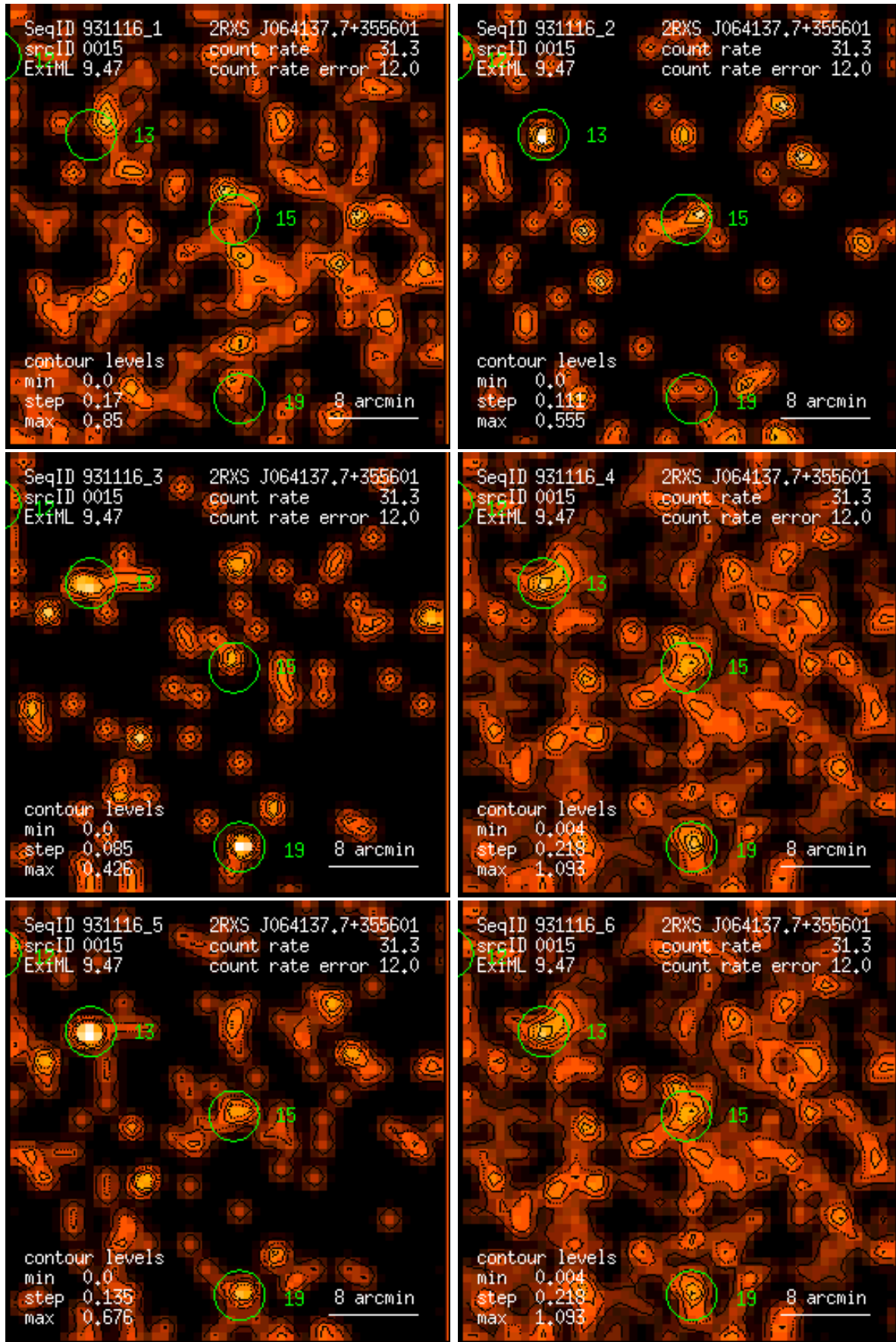
Figure 15: RASS 931116: detection 0015: band rate images, Gaussian filter: (1) PSPC channels 11 – 41, (2) 52 – 90, (3) 91 – 201, (4) 11 – 235, (5) 52 – 201, (6) 11 – 201. Broad band rates in counts/ks. Band rate contour levels in counts/ks/arcmin 2 .
