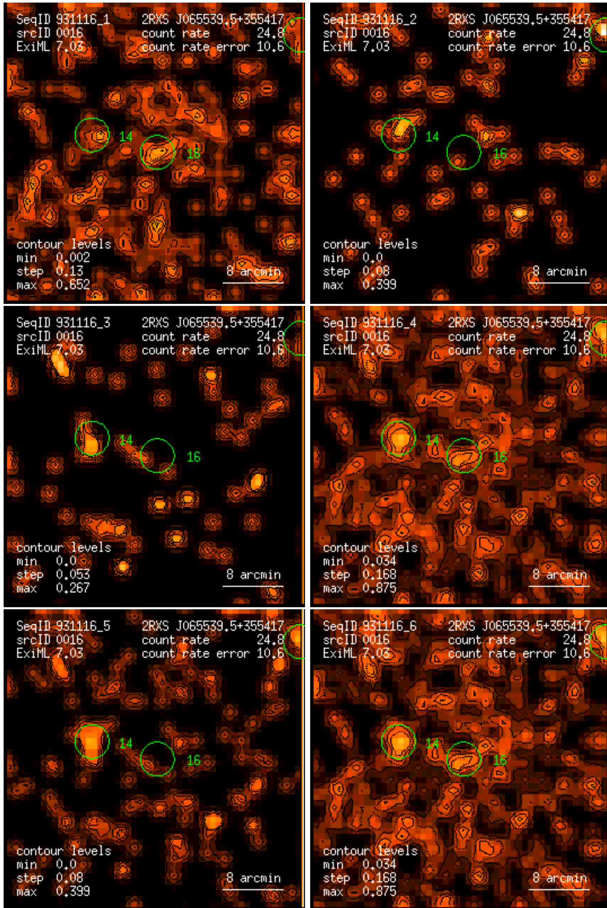
Figure 16: RASS 931116: detection 0016: band rate images, Gaussian filter: (1) PSPC channels 11 – 41, (2) 52 – 90, (3) 91 – 201, (4) 11 – 235, (5) 52 – 201, (6) 11 – 201. Broad band rates in counts/ks. Band rate contour levels in counts/ks/arcmin 2 .
