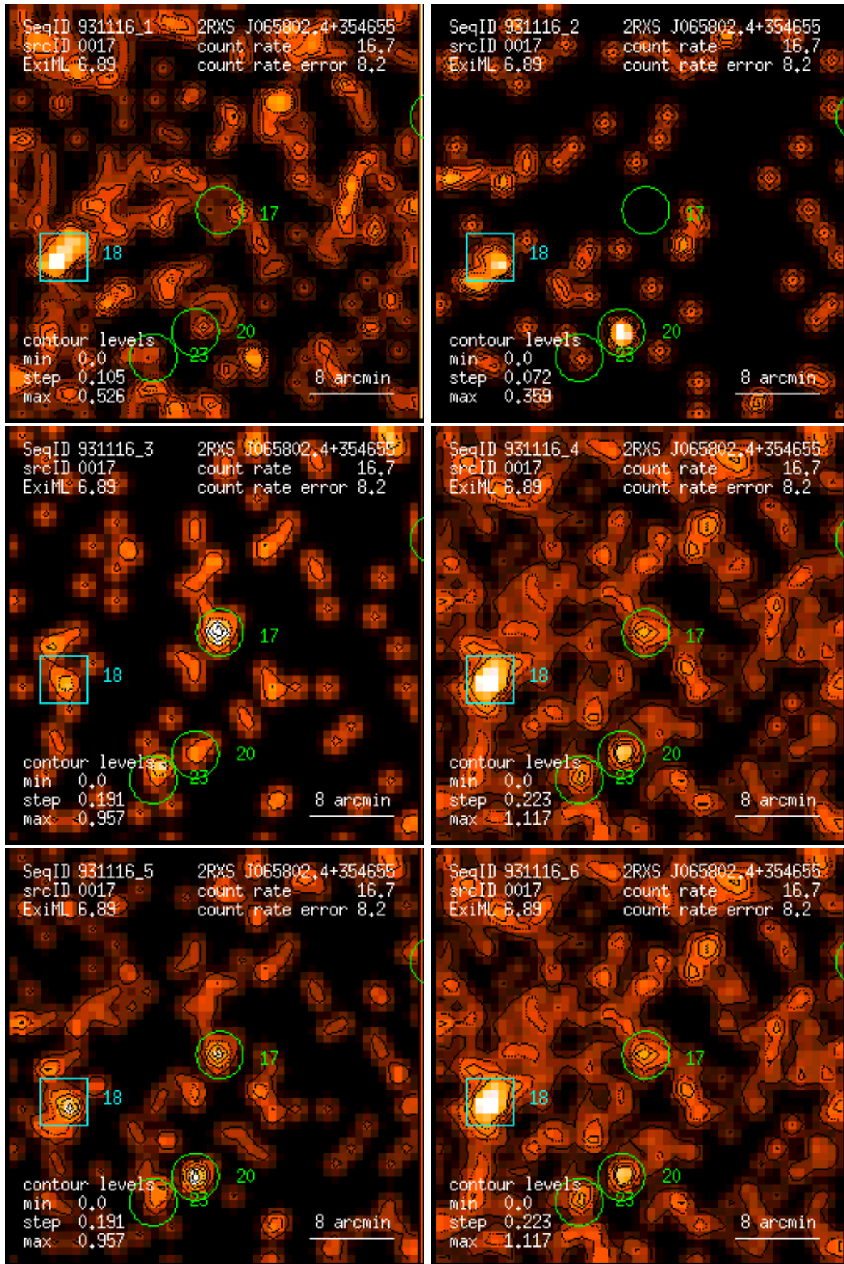
Figure 17: RASS 931116: detection 0017: band rate images, Gaussian filter: (1) PSPC channels 11 – 41, (2) 52 – 90, (3) 91 – 201, (4) 11 – 235, (5) 52 – 201, (6) 11 – 201. Broad band rates in counts/ks. Band rate contour levels in counts/ks/arcmin 2 .
