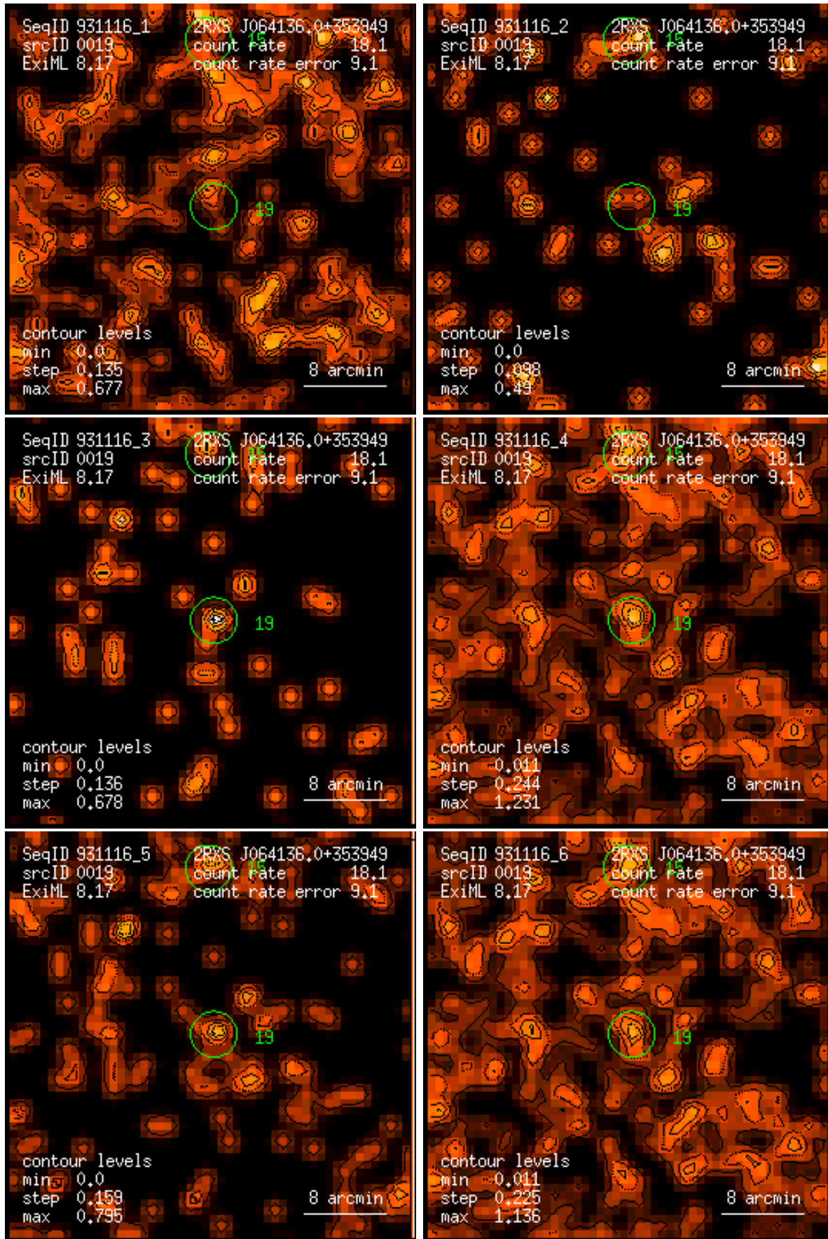
Figure 19: RASS 931116: detection 0019: band rate images, Gaussian filter: (1) PSPC channels 11 – 41, (2) 52 – 90, (3) 91 – 201, (4) 11 – 235, (5) 52 – 201, (6) 11 – 201. Broad band rates in counts/ks. Band rate contour levels in counts/ks/arcmin 2 .
