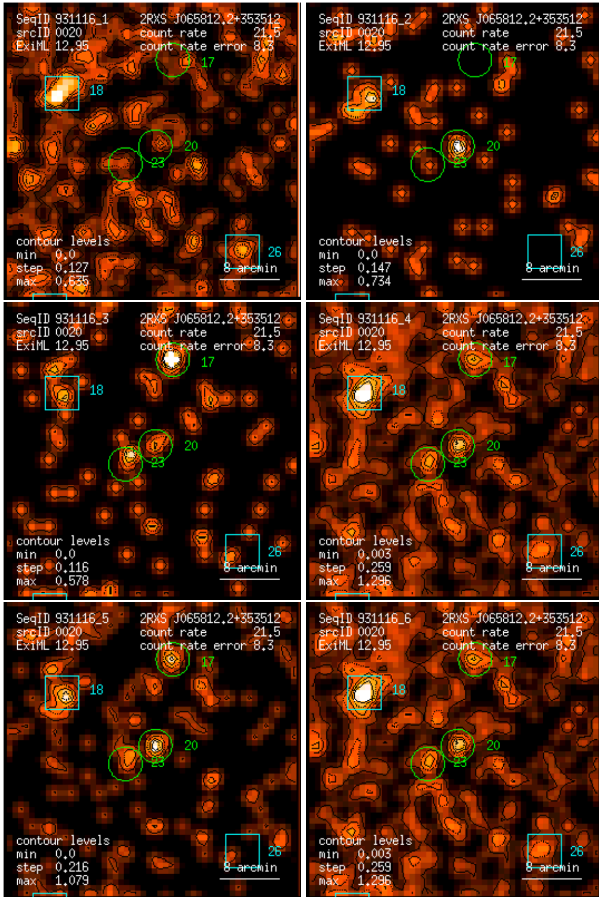
Figure 20: RASS 931116: detection 0020: band rate images, Gaussian filter: (1) PSPC channels 11 – 41, (2) 52 – 90, (3) 91 – 201, (4) 11 – 235, (5) 52 – 201, (6) 11 – 201. Broad band rates in counts/ks. Band rate contour levels in counts/ks/arcmin 2 .
