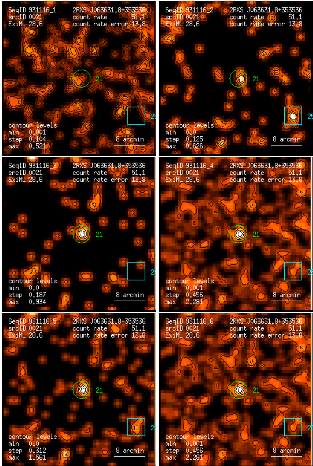
Figure 21: RASS 931116: detection 0021: band rate images, Gaussian filter: (1) PSPC channels 11 – 41, (2) 52 – 90, (3) 91 – 201, (4) 11 – 235, (5) 52 – 201, (6) 11 – 201. Broad band rates in counts/ks. Band rate contour levels in counts/ks/arcmin 2 .
