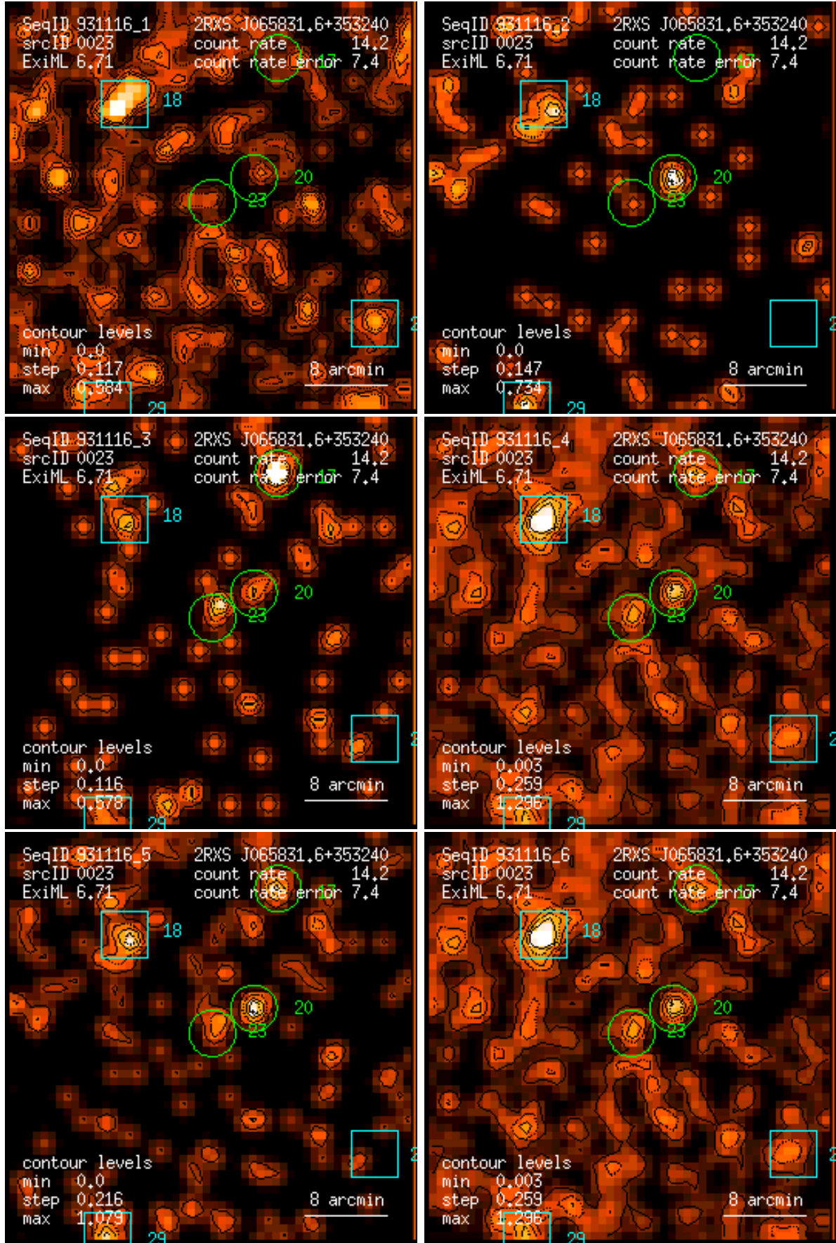
Figure 23: RASS 931116: detection 0023: band rate images, Gaussian filter: (1) PSPC channels 11 – 41, (2) 52 – 90, (3) 91 – 201, (4) 11 – 235, (5) 52 – 201, (6) 11 – 201. Broad band rates in counts/ks. Band rate contour levels in counts/ks/arcmin 2 .
