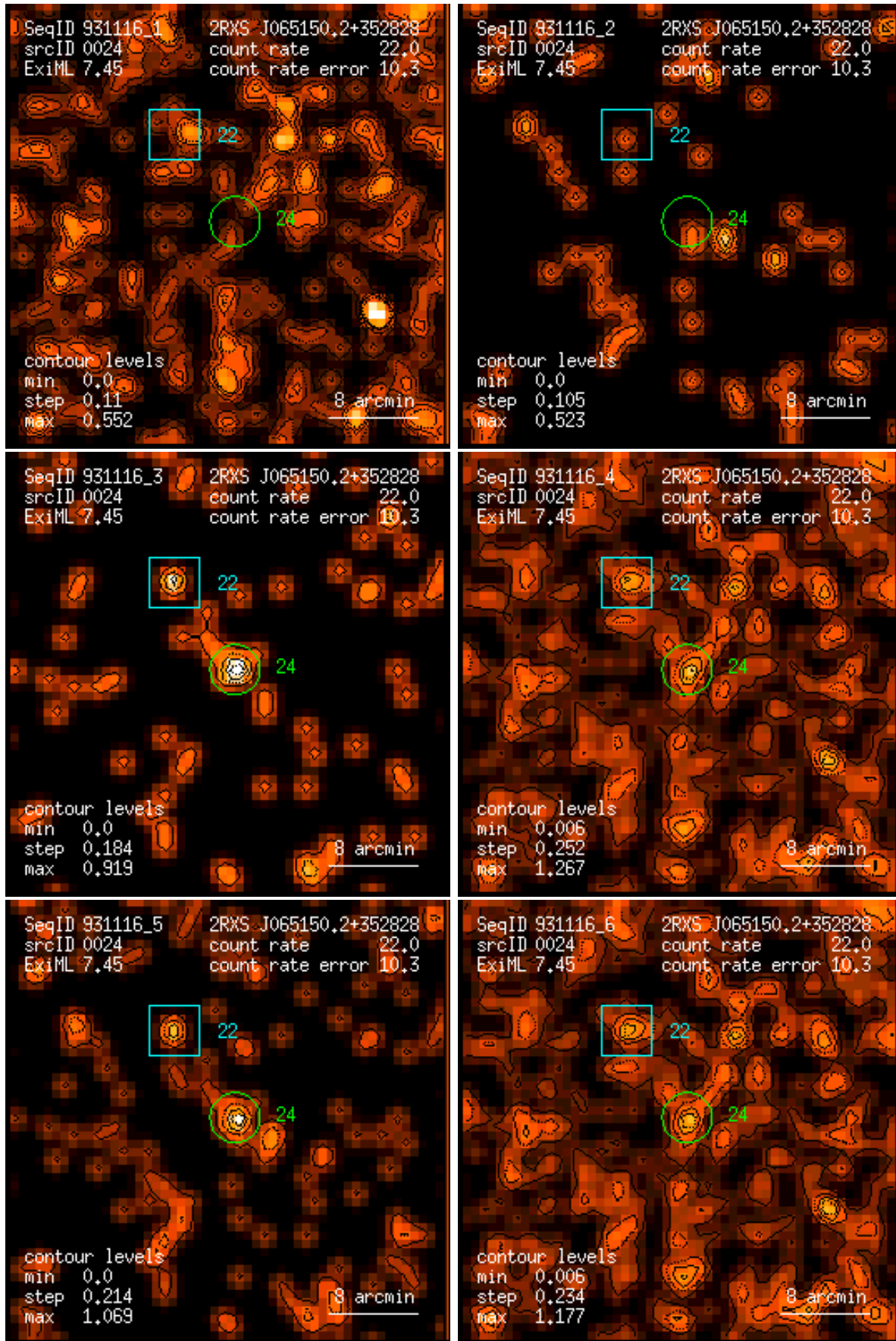
Figure 24: RASS 931116: detection 0024: band rate images, Gaussian filter: (1) PSPC channels 11 – 41, (2) 52 – 90, (3) 91 – 201, (4) 11 – 235, (5) 52 – 201, (6) 11 – 201. Broad band rates in counts/ks. Band rate contour levels in counts/ks/arcmin 2 .
