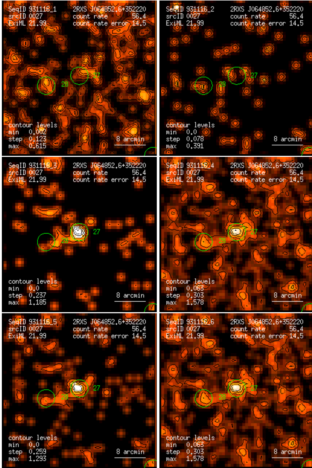
Figure 27: RASS 931116: detection 0027: band rate images, Gaussian filter: (1) PSPC channels 11 – 41, (2) 52 – 90, (3) 91 – 201, (4) 11 – 235, (5) 52 – 201, (6) 11 – 201. Broad band rates in counts/ks. Band rate contour levels in counts/ks/arcmin 2 .
