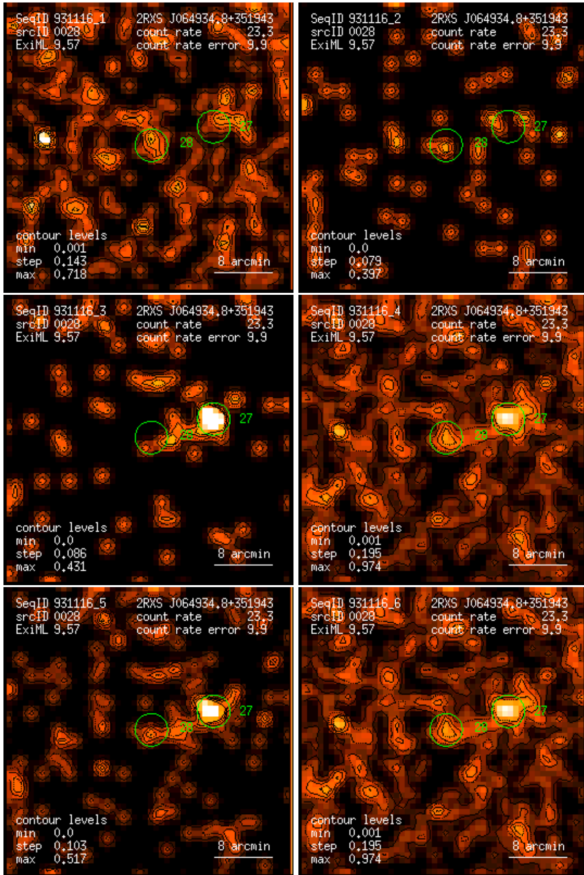
Figure 28: RASS 931116: detection 0028: band rate images, Gaussian filter: (1) PSPC channels 11 – 41, (2) 52 – 90, (3) 91 – 201, (4) 11 – 235, (5) 52 – 201, (6) 11 – 201. Broad band rates in counts/ks. Band rate contour levels in counts/ks/arcmin 2 .
