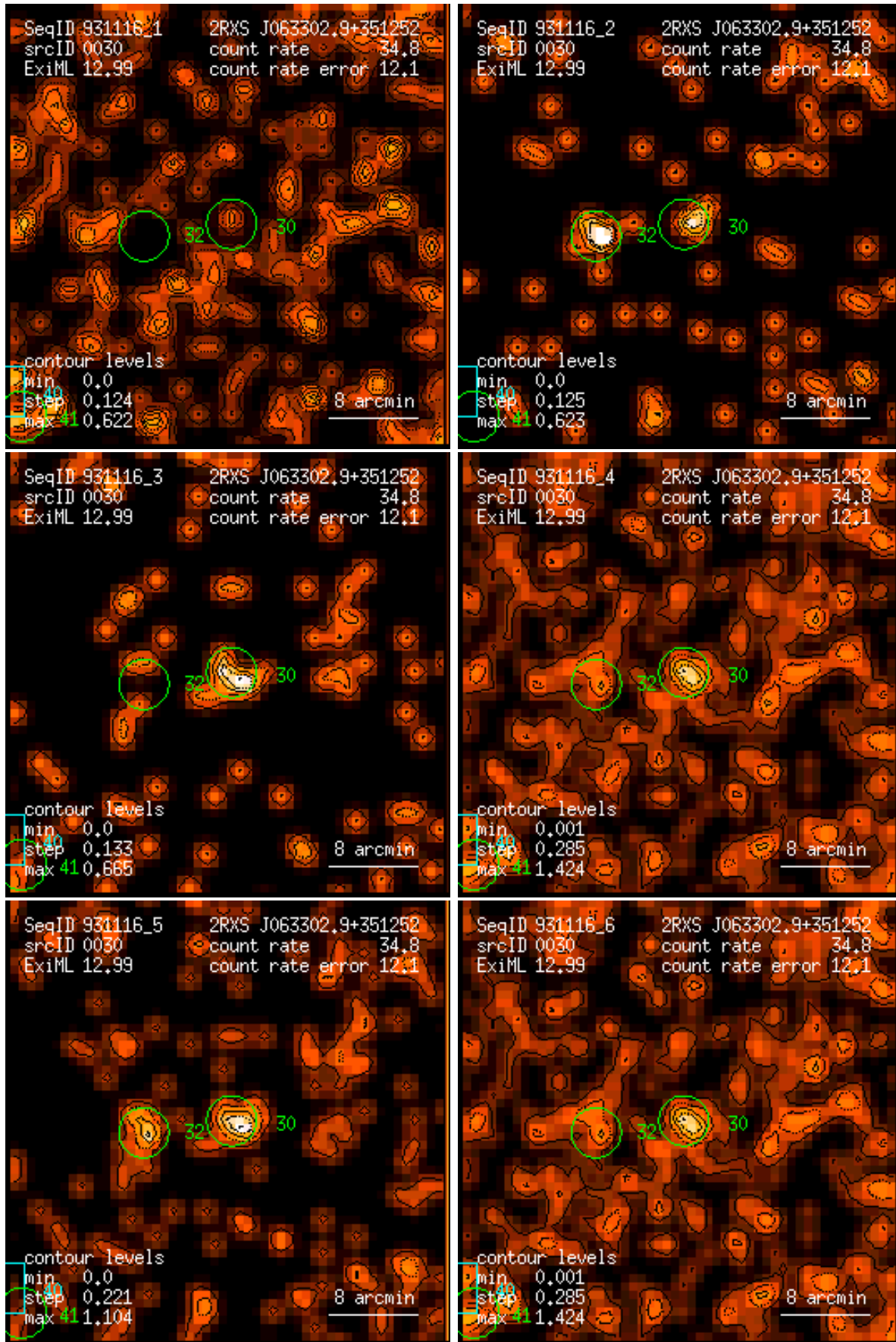
Figure 30: RASS 931116: detection 0030: band rate images, Gaussian filter: (1) PSPC channels 11 – 41, (2) 52 – 90, (3) 91 – 201, (4) 11 – 235, (5) 52 – 201, (6) 11 – 201. Broad band rates in counts/ks. Band rate contour levels in counts/ks/arcmin 2 .
