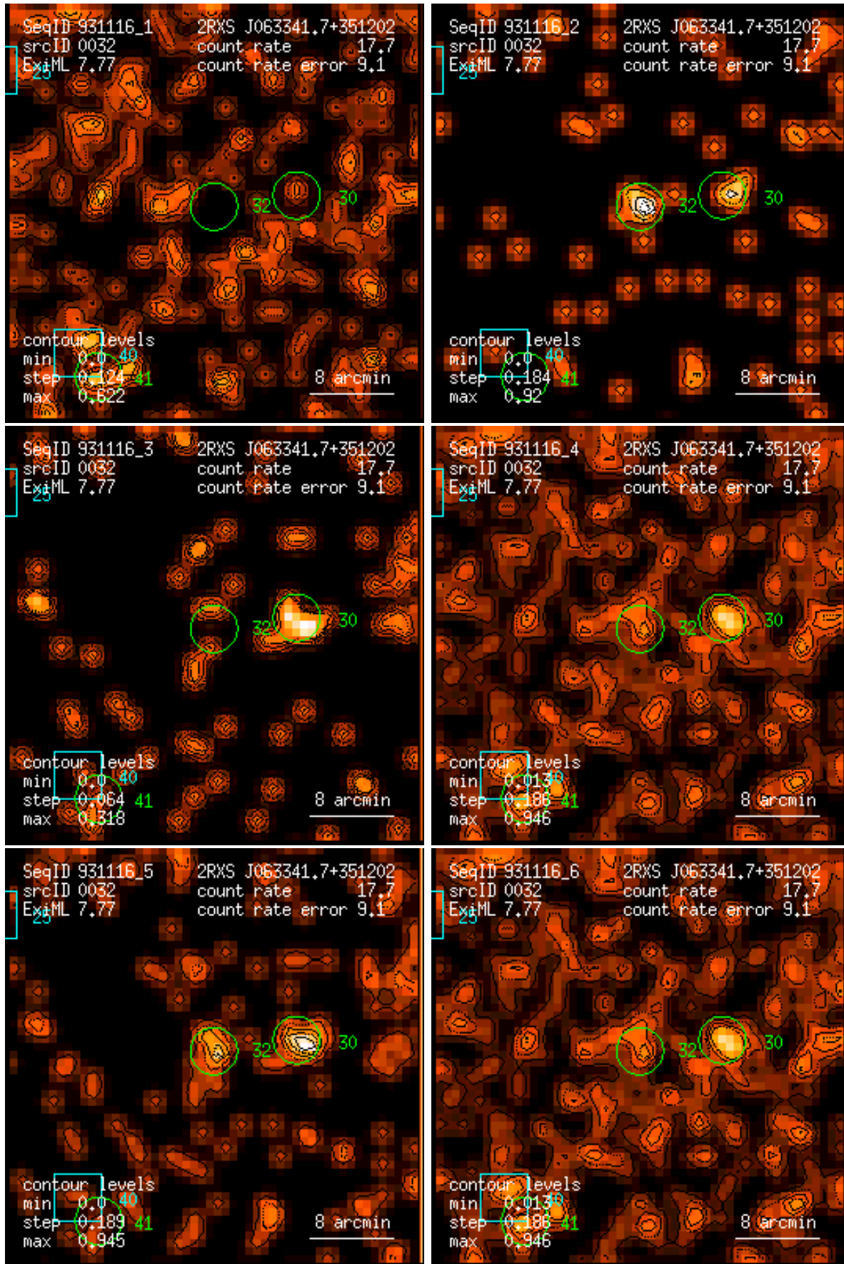
Figure 32: RASS 931116: detection 0032: band rate images, Gaussian filter: (1) PSPC channels 11 – 41, (2) 52 – 90, (3) 91 – 201, (4) 11 – 235, (5) 52 – 201, (6) 11 – 201. Broad band rates in counts/ks. Band rate contour levels in counts/ks/arcmin 2 .
