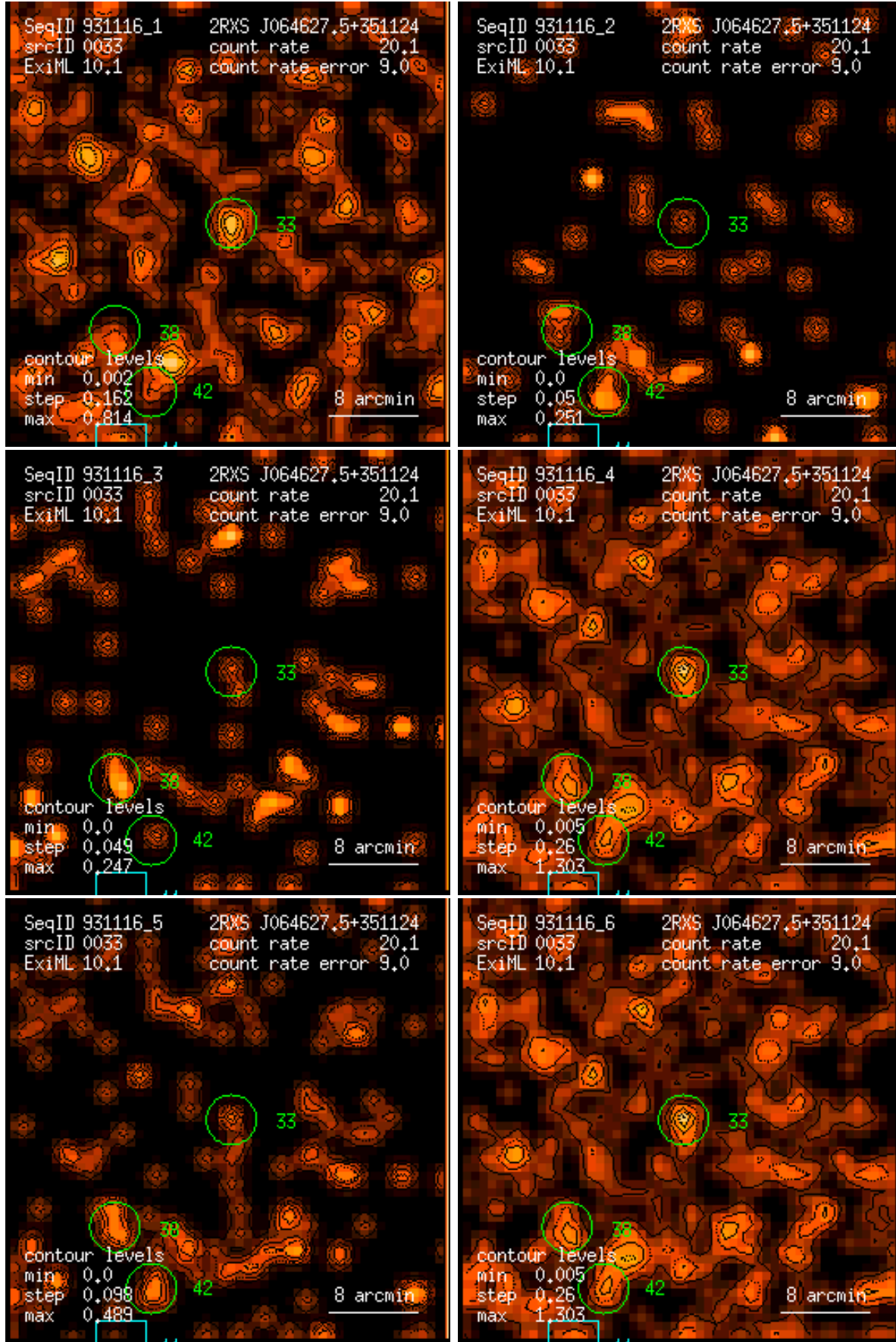
Figure 33: RASS 931116: detection 0033: band rate images, Gaussian filter: (1) PSPC channels 11 – 41, (2) 52 – 90, (3) 91 – 201, (4) 11 – 235, (5) 52 – 201, (6) 11 – 201. Broad band rates in counts/ks. Band rate contour levels in counts/ks/arcmin 2 .
