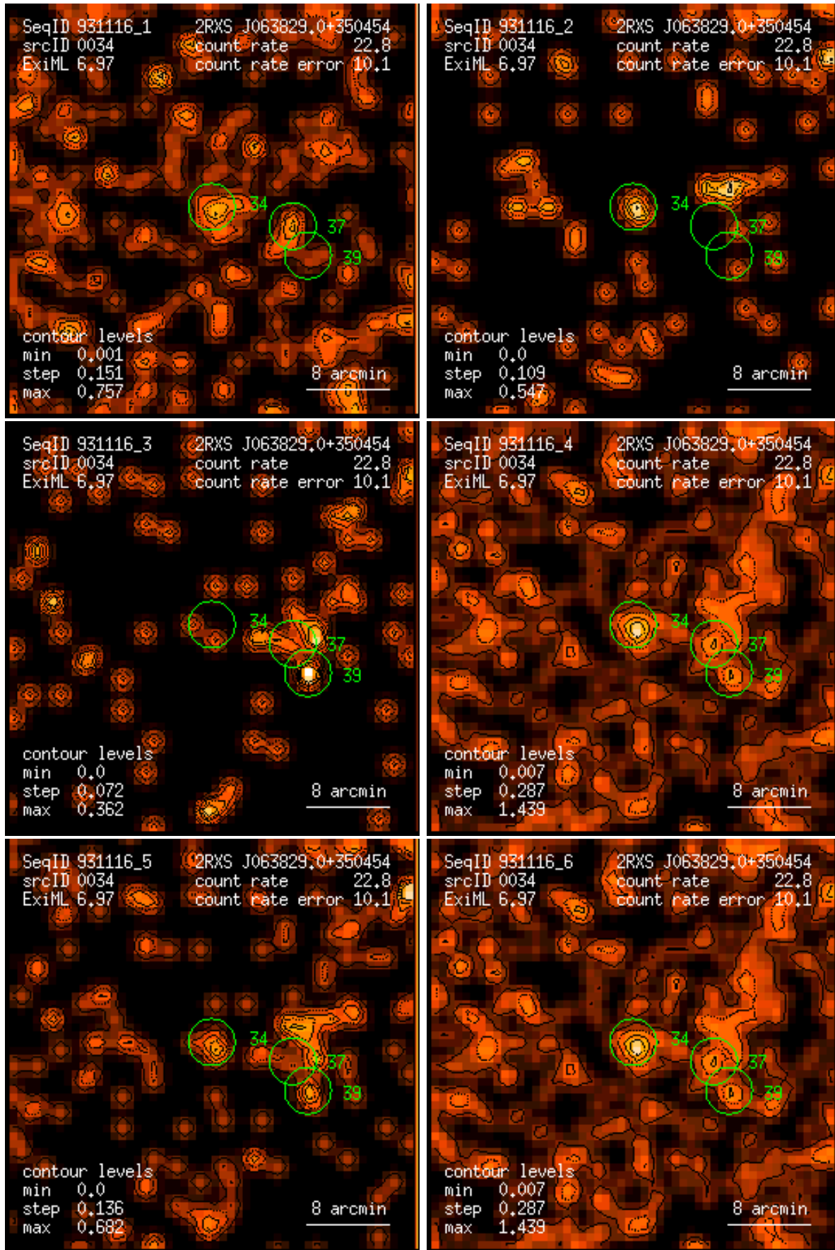
Figure 34: RASS 931116: detection 0034: band rate images, Gaussian filter: (1) PSPC channels 11 – 41, (2) 52 – 90, (3) 91 – 201, (4) 11 – 235, (5) 52 – 201, (6) 11 – 201. Broad band rates in counts/ks. Band rate contour levels in counts/ks/arcmin 2 .
