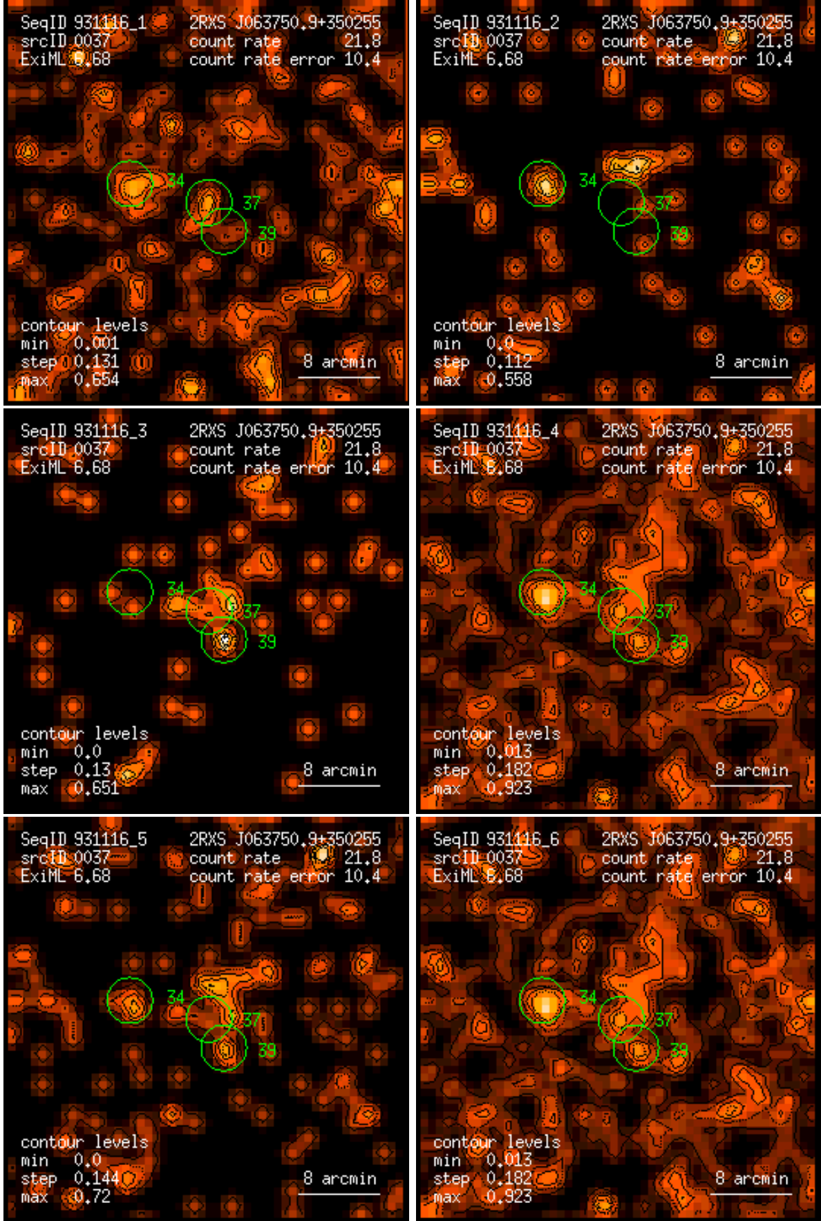
Figure 37: RASS 931116: detection 0037: band rate images, Gaussian filter: (1) PSPC channels 11 – 41, (2) 52 – 90, (3) 91 – 201, (4) 11 – 235, (5) 52 – 201, (6) 11 – 201. Broad band rates in counts/ks. Band rate contour levels in counts/ks/arcmin 2 .
