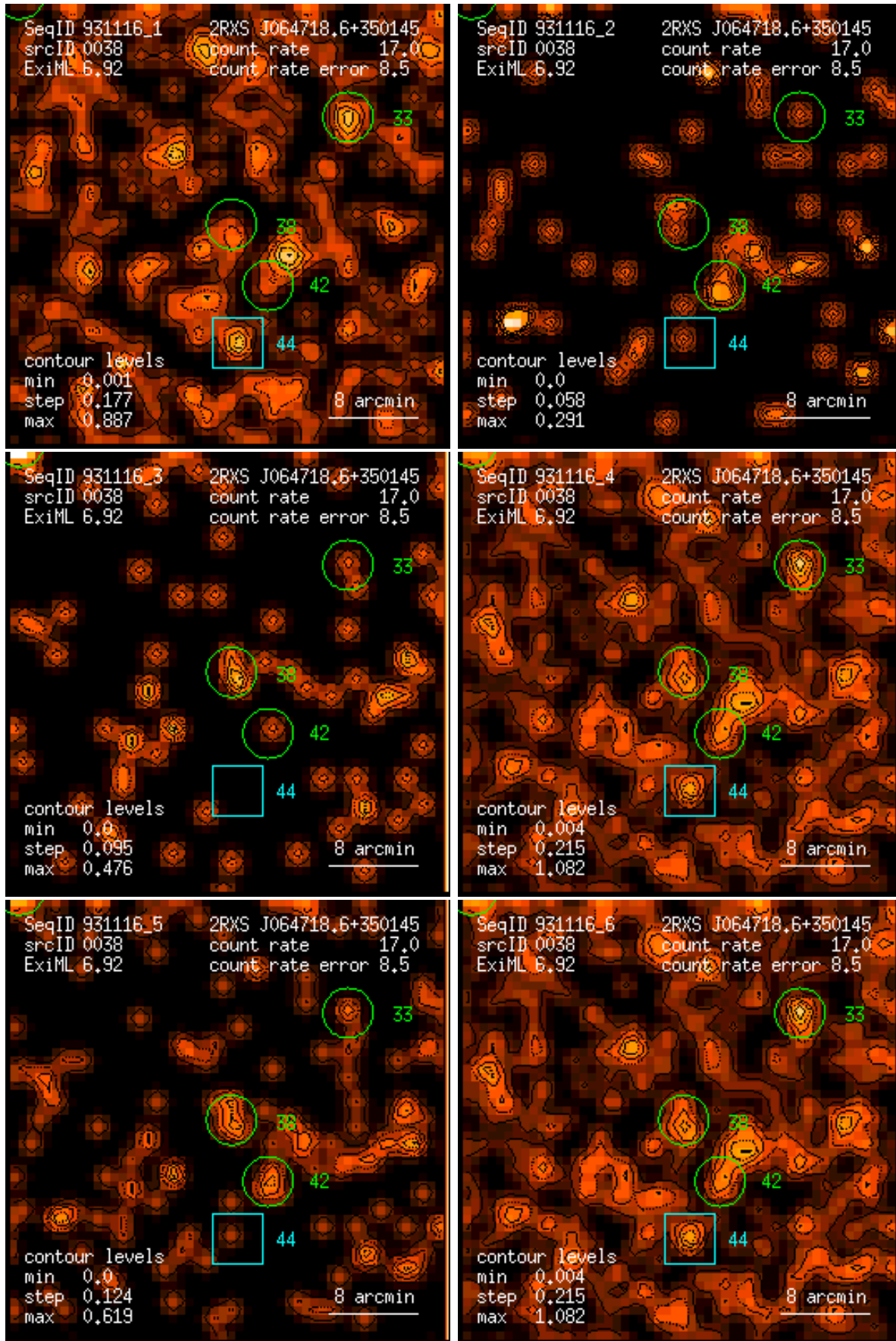
Figure 38: RASS 931116: detection 0038: band rate images, Gaussian filter: (1) PSPC channels 11 – 41, (2) 52 – 90, (3) 91 – 201, (4) 11 – 235, (5) 52 – 201, (6) 11 – 201. Broad band rates in counts/ks. Band rate contour levels in counts/ks/arcmin 2 .
