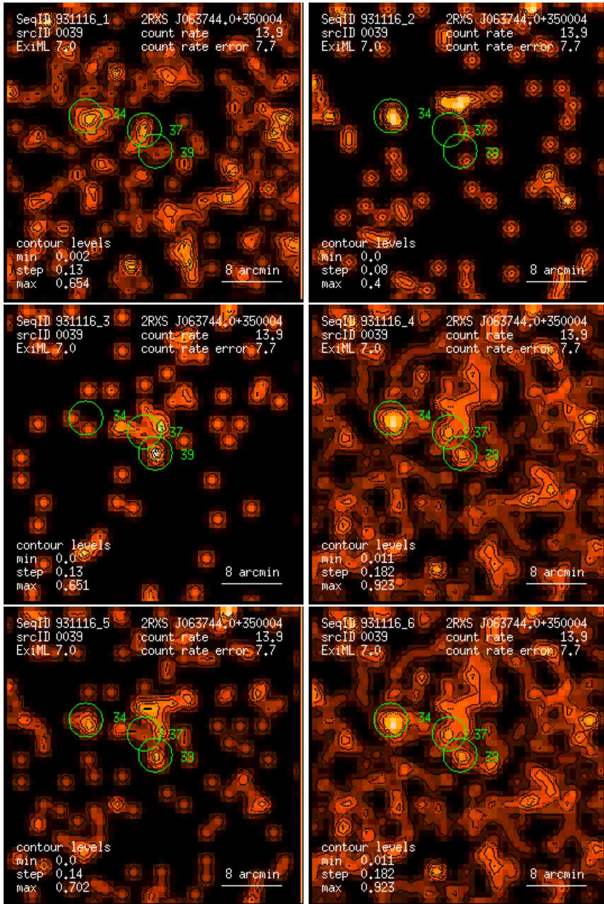
Figure 39: RASS 931116: detection 0039: band rate images, Gaussian filter: (1) PSPC channels 11 – 41, (2) 52 – 90, (3) 91 – 201, (4) 11 – 235, (5) 52 – 201, (6) 11 – 201. Broad band rates in counts/ks. Band rate contour levels in counts/ks/arcmin 2 .
