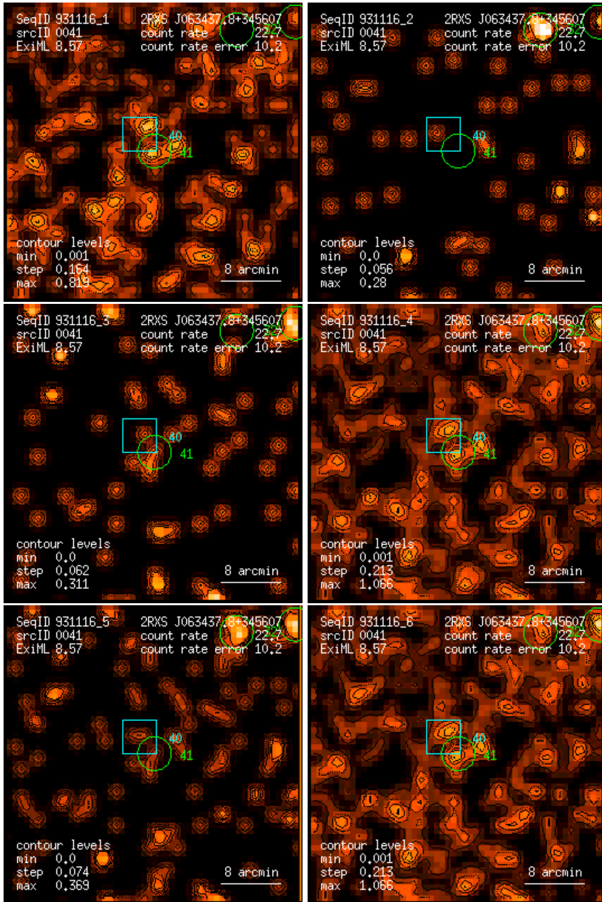
Figure 41: RASS 931116: detection 0041: band rate images, Gaussian filter: (1) PSPC channels 11 – 41, (2) 52 – 90, (3) 91 – 201, (4) 11 – 235, (5) 52 – 201, (6) 11 – 201. Broad band rates in counts/ks. Band rate contour levels in counts/ks/arcmin 2 .
