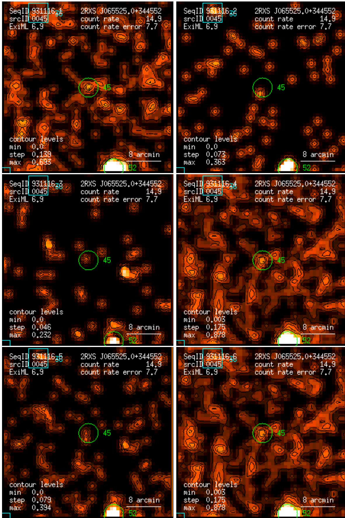
Figure 45: RASS 931116: detection 0045: band rate images, Gaussian filter: (1) PSPC channels 11 – 41, (2) 52 – 90, (3) 91 – 201, (4) 11 – 235, (5) 52 – 201, (6) 11 – 201. Broad band rates in counts/ks. Band rate contour levels in counts/ks/arcmin 2 .
