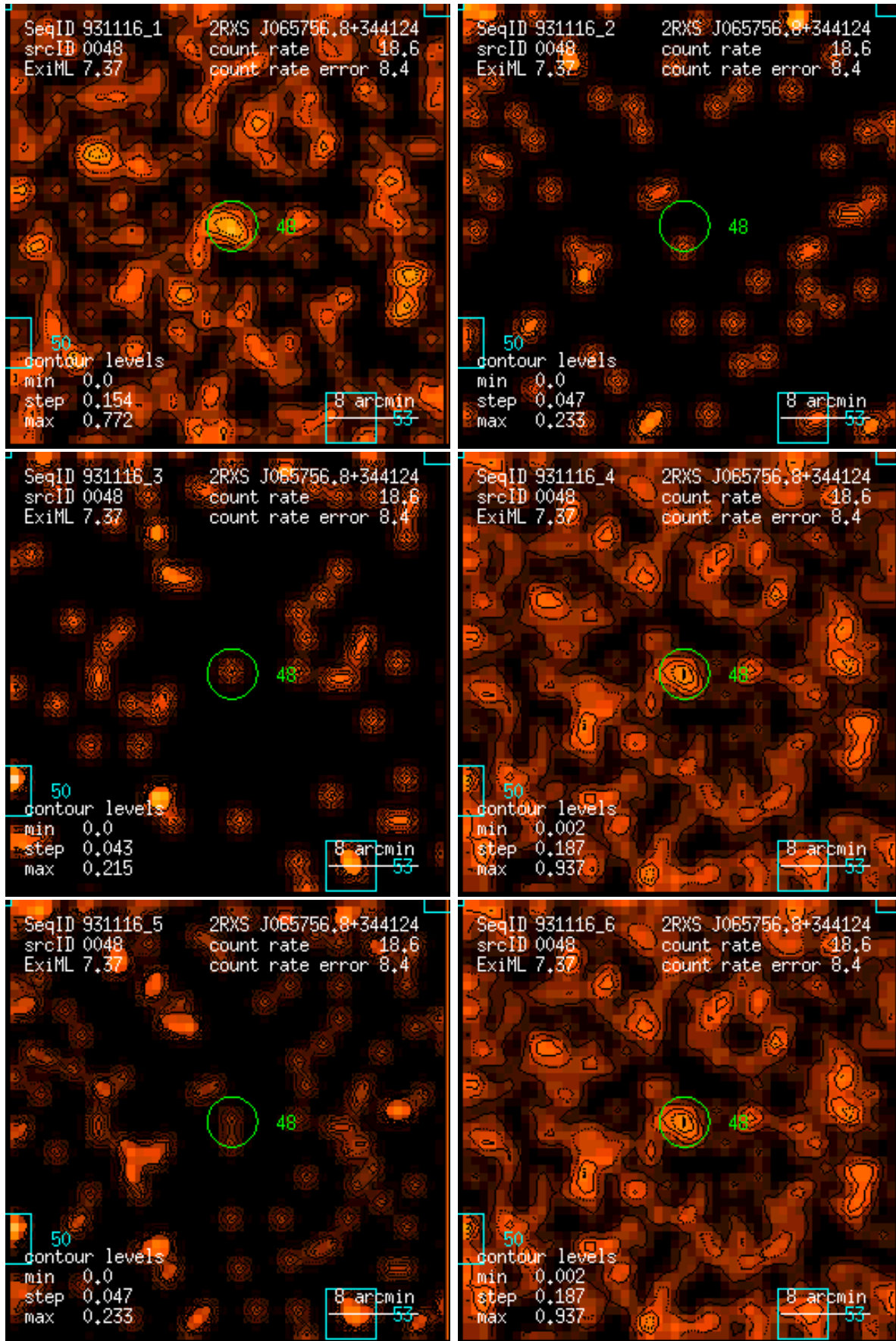
Figure 48: RASS 931116: detection 0048: band rate images, Gaussian filter: (1) PSPC channels 11 – 41, (2) 52 – 90, (3) 91 – 201, (4) 11 – 235, (5) 52 – 201, (6) 11 – 201. Broad band rates in counts/ks. Band rate contour levels in counts/ks/arcmin 2 .
