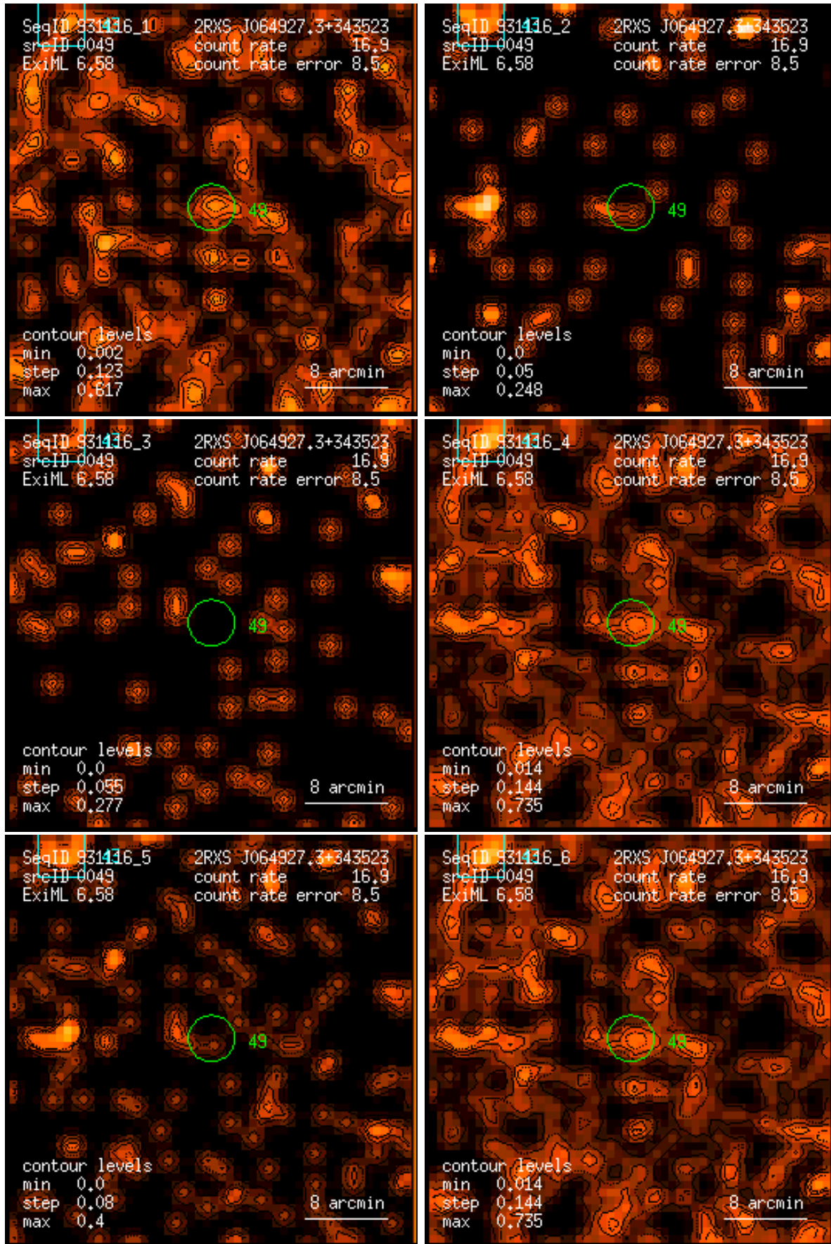
Figure 49: RASS 931116: detection 0049: band rate images, Gaussian filter: (1) PSPC channels 11 – 41, (2) 52 – 90, (3) 91 – 201, (4) 11 – 235, (5) 52 – 201, (6) 11 – 201. Broad band rates in counts/ks. Band rate contour levels in counts/ks/arcmin 2 .
