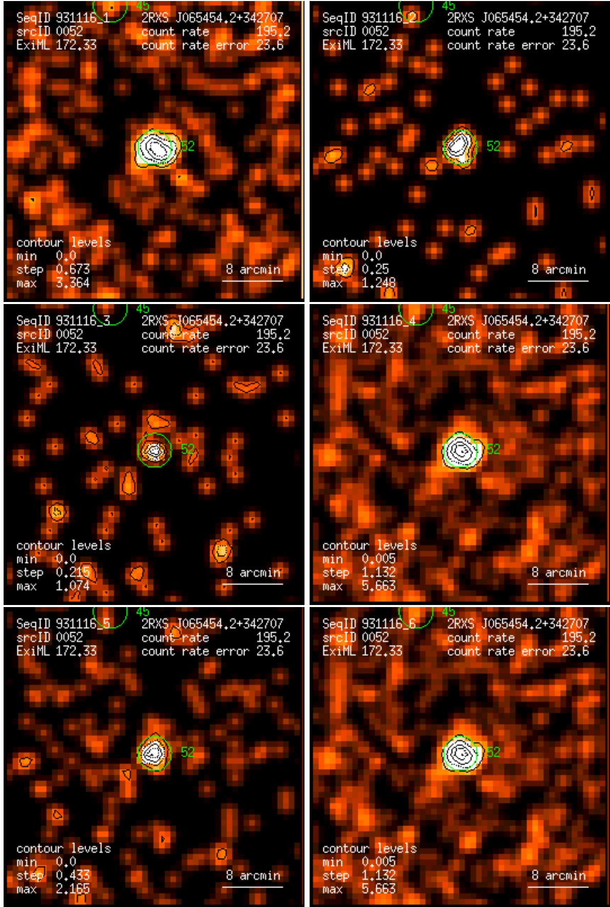
Figure 52: RASS 931116: detection 0052: band rate images, Gaussian filter: (1) PSPC channels 11 – 41, (2) 52 – 90, (3) 91 – 201, (4) 11 – 235, (5) 52 – 201, (6) 11 – 201. Broad band rates in counts/ks. Band rate contour levels in counts/ks/arcmin 2 .
