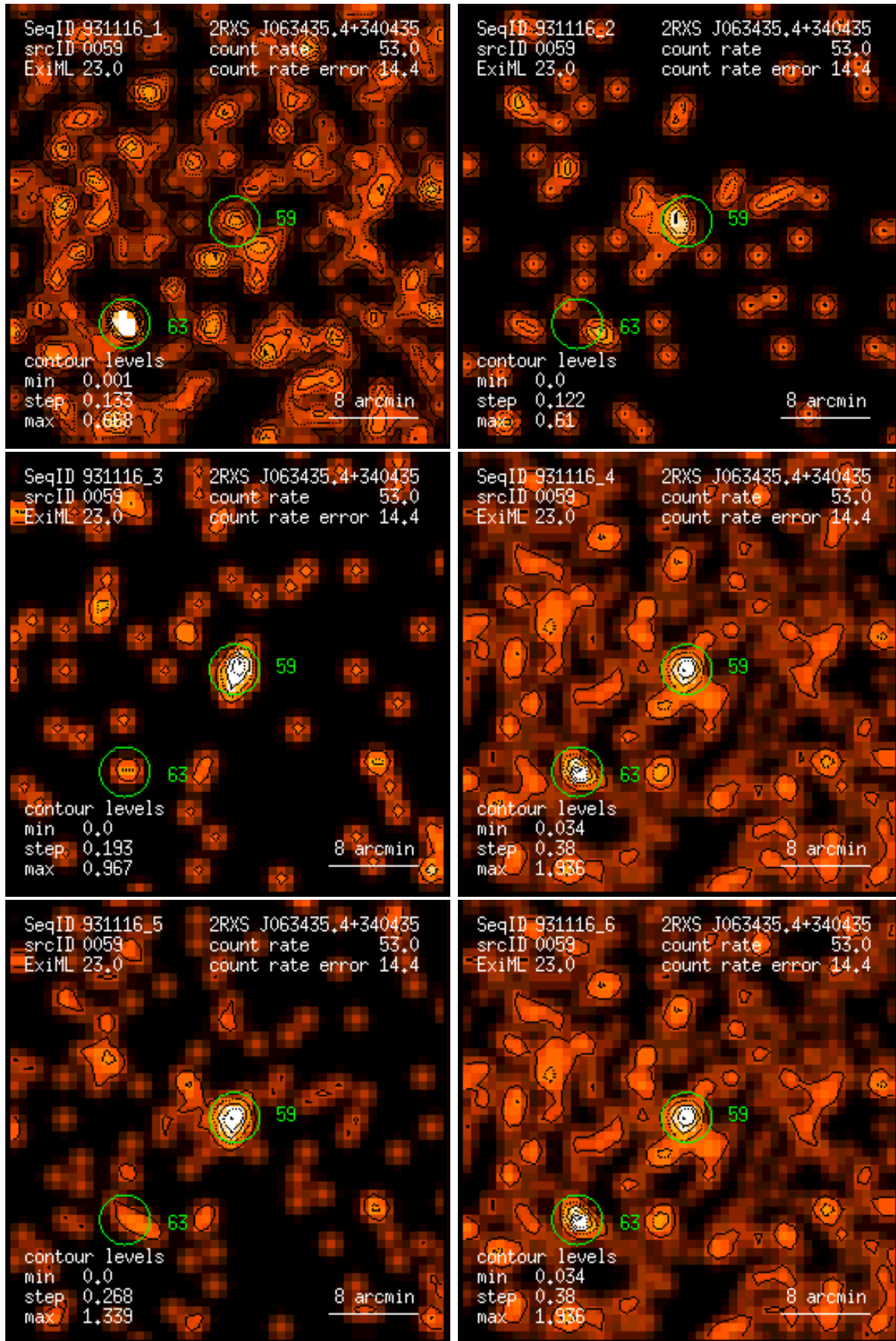
Figure 59: RASS 931116: detection 0059: band rate images, Gaussian filter: (1) PSPC channels 11 – 41, (2) 52 – 90, (3) 91 – 201, (4) 11 – 235, (5) 52 – 201, (6) 11 – 201. Broad band rates in counts/ks. Band rate contour levels in counts/ks/arcmin 2 .
