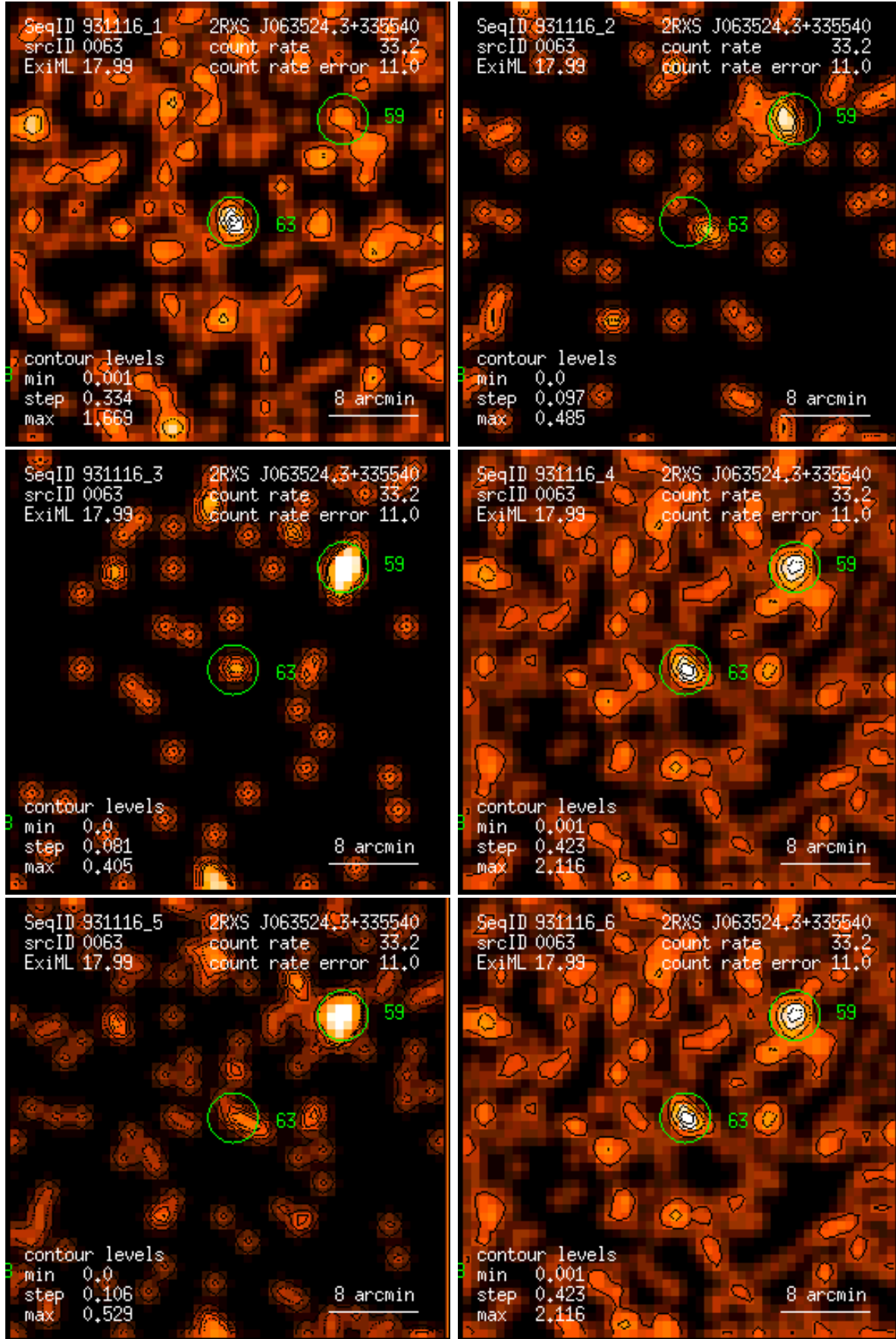
Figure 63: RASS 931116: detection 0063: band rate images, Gaussian filter: (1) PSPC channels 11 – 41, (2) 52 – 90, (3) 91 – 201, (4) 11 – 235, (5) 52 – 201, (6) 11 – 201. Broad band rates in counts/ks. Band rate contour levels in counts/ks/arcmin 2 .
