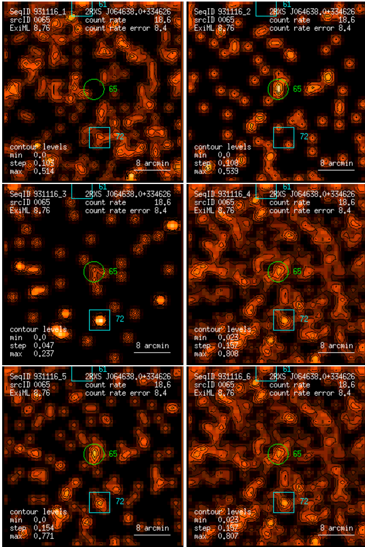
Figure 65: RASS 931116: detection 0065: band rate images, Gaussian filter: (1) PSPC channels 11 – 41, (2) 52 – 90, (3) 91 – 201, (4) 11 – 235, (5) 52 – 201, (6) 11 – 201. Broad band rates in counts/ks. Band rate contour levels in counts/ks/arcmin 2 .
