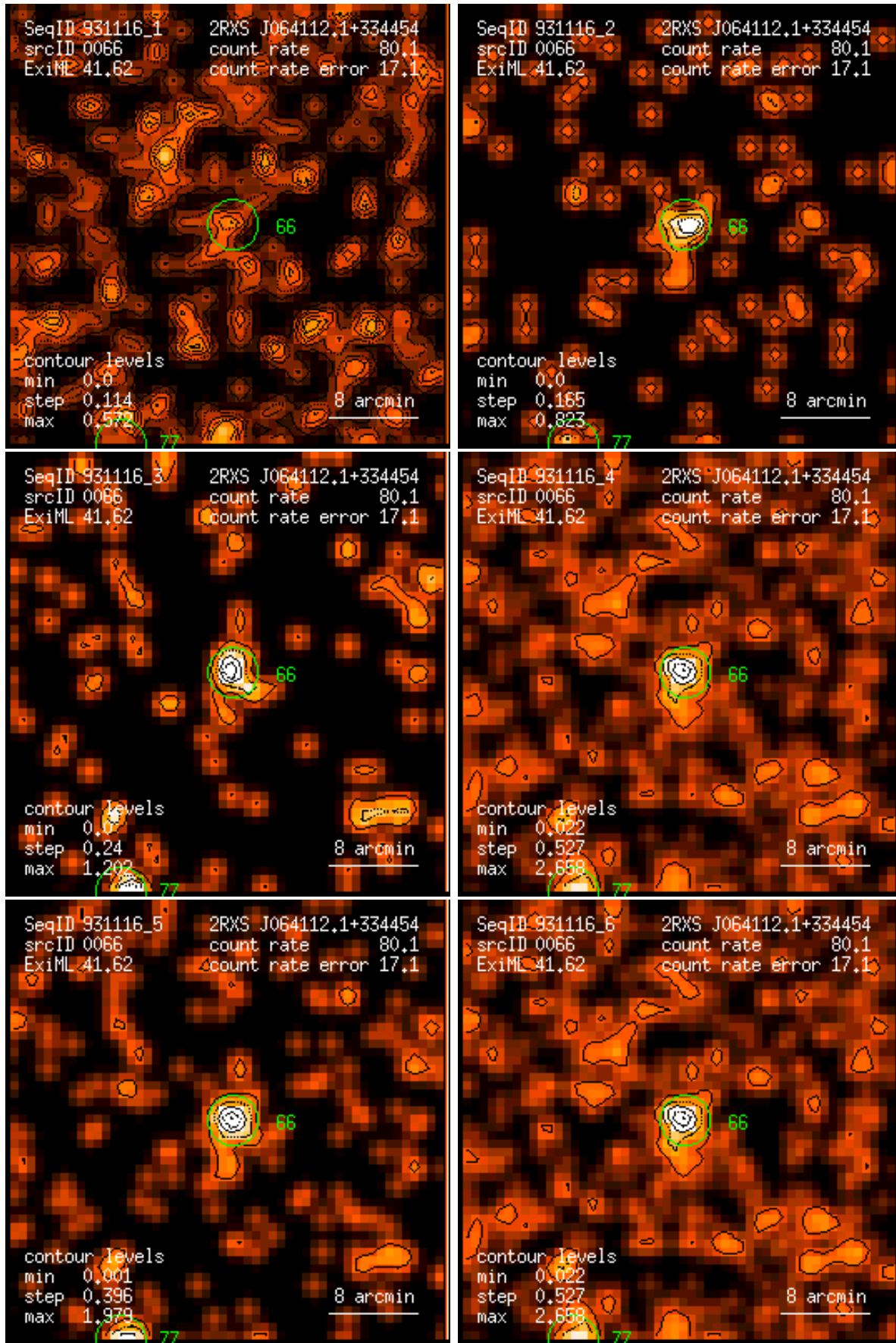
Figure 66: RASS 931116: detection 0066: band rate images, Gaussian filter: (1) PSPC channels 11 – 41, (2) 52 – 90, (3) 91 – 201, (4) 11 – 235, (5) 52 – 201, (6) 11 – 201. Broad band rates in counts/ks. Band rate contour levels in counts/ks/arcmin 2 .
